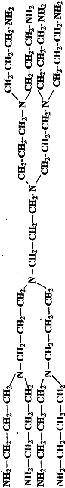
Polypropyleneimine Dendrimer-8
