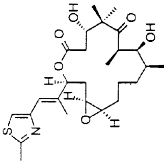
epothilone A
