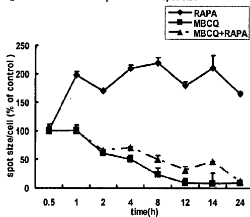
b HCS assay of GFP-LC3 spot size
