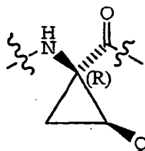
Q syn to nitrogen
