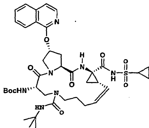
Compound 150
