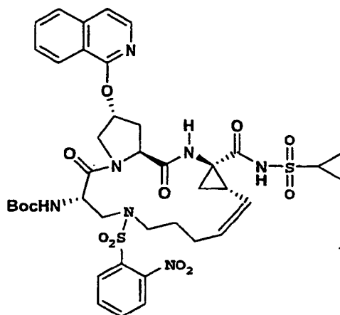
compound 145
