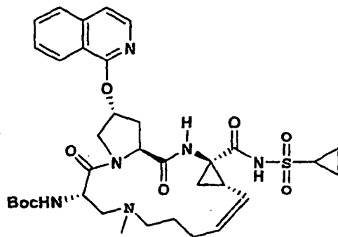
Compound 147
