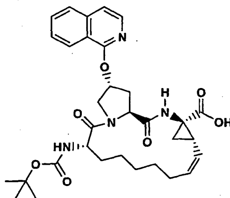
Example 2, Compound 1
