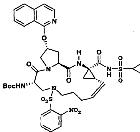
Compound 145
