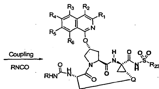
Compounds of Formula I
