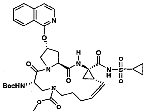
Compound 148
