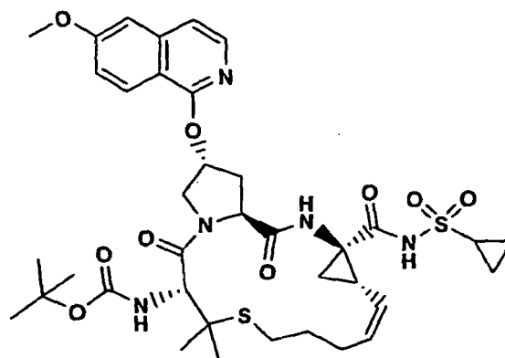
Compound 80
