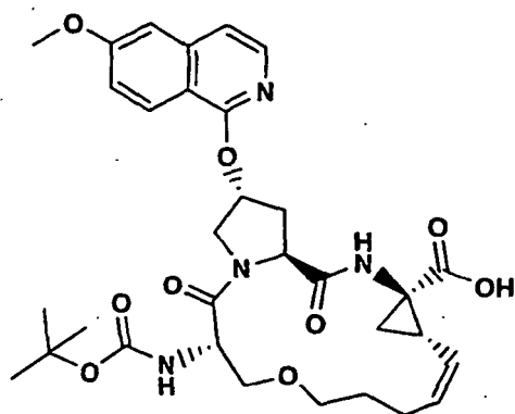
Compound 84
