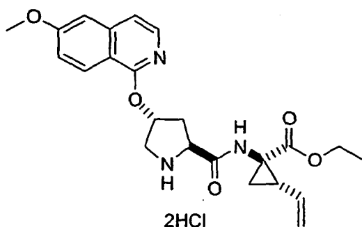
Example 22
