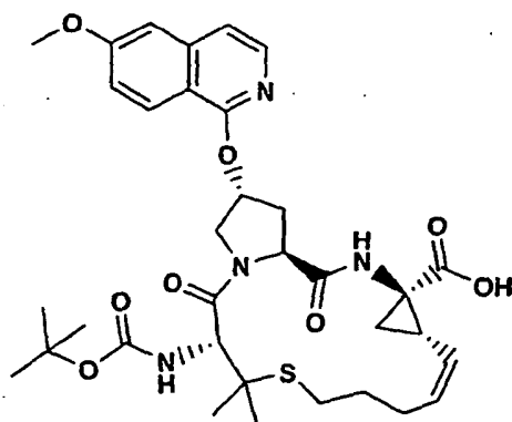
Compound 79
