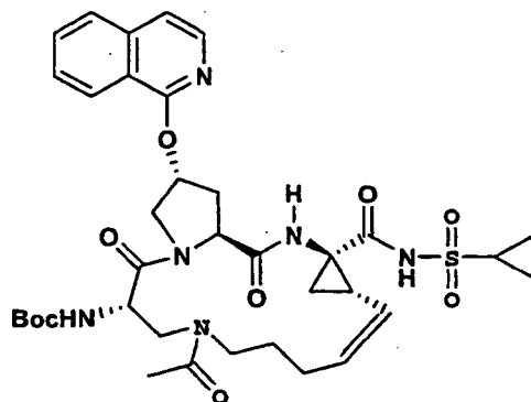
Compound 146
