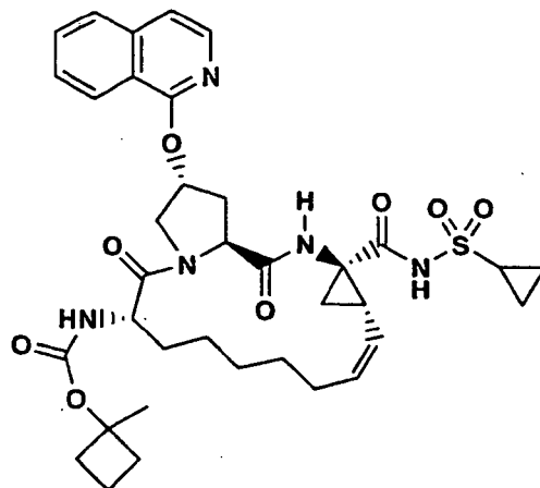
compound 56
