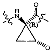
Q syn to carbonyl
