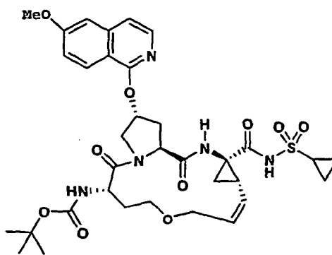
compound 141
