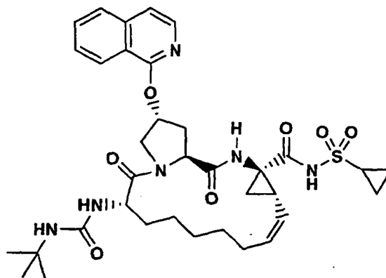
compound 126
