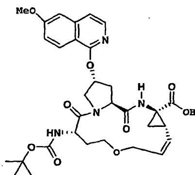
compound 140
