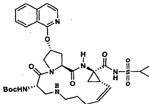
Compound 151
