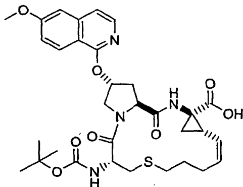
Compound 18A
