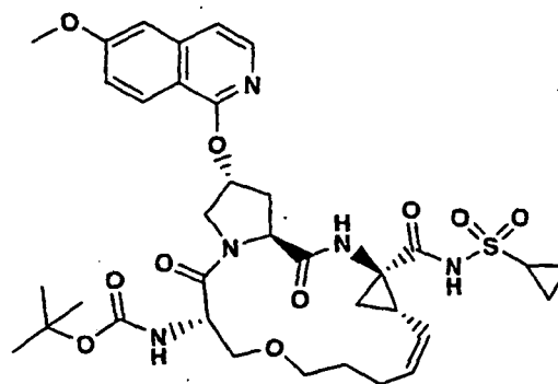
Compound 85
