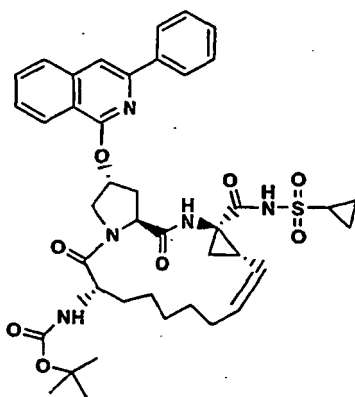
compound 58
