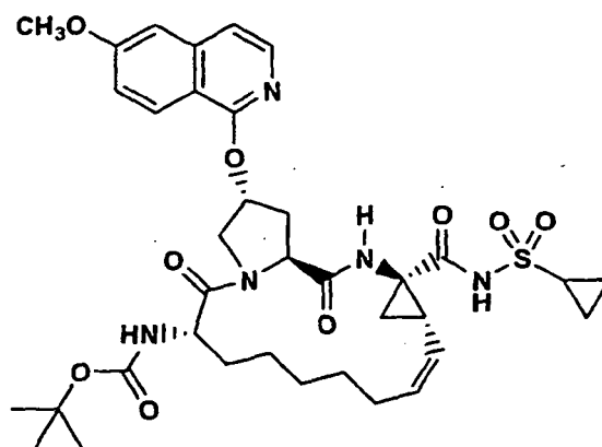
Compound 17B
