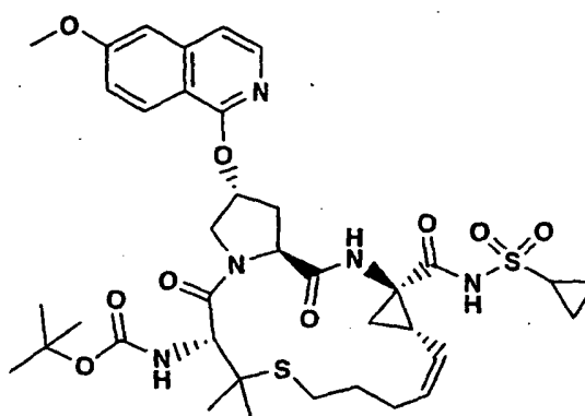
Compound 80
