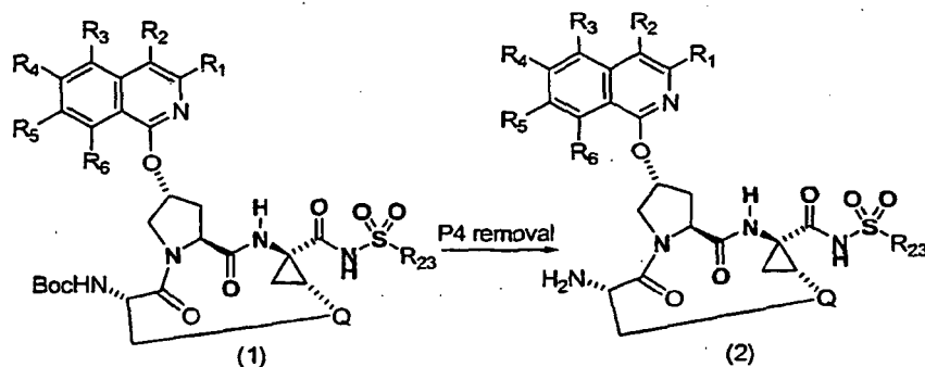
Compounds of Formula I
