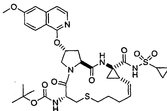
Compound 18B
