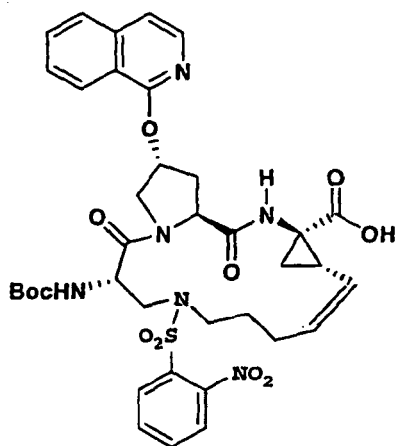
Compound 144
