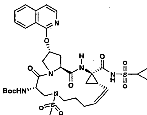
Compound 153
