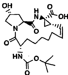
Example 20
