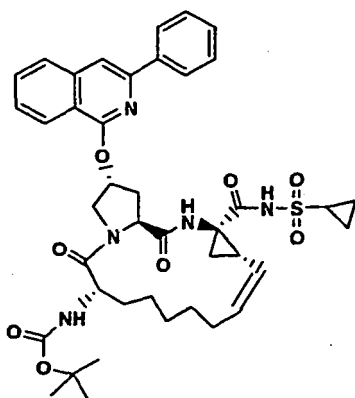
compound 58
