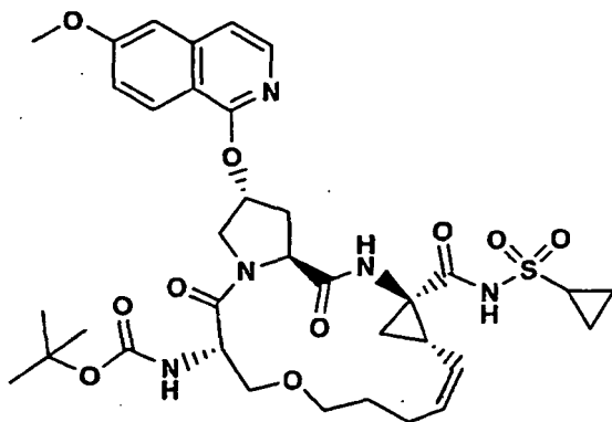
Compound 85
