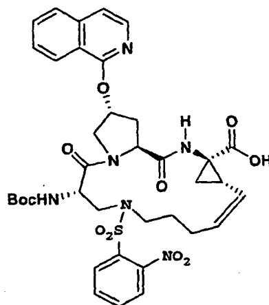
compound 144
