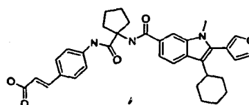
Replicase Inhibitor Compound Y, WO 03/010141
