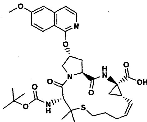
Compound 79
