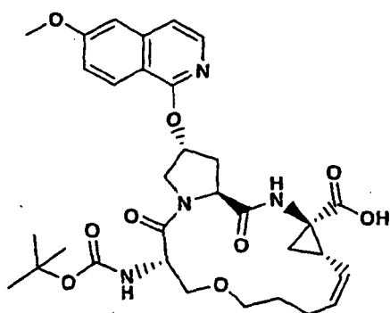
Compound 84
