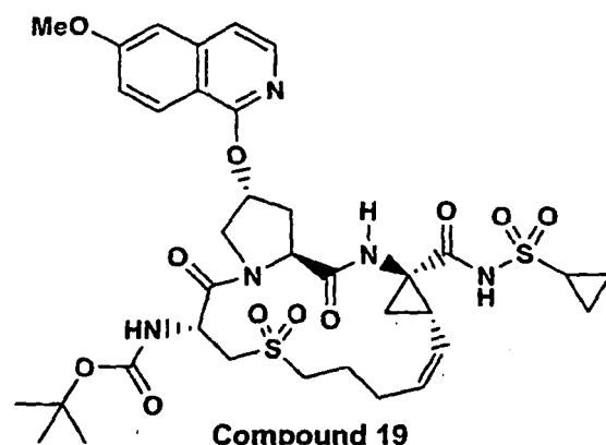
Compound 19
