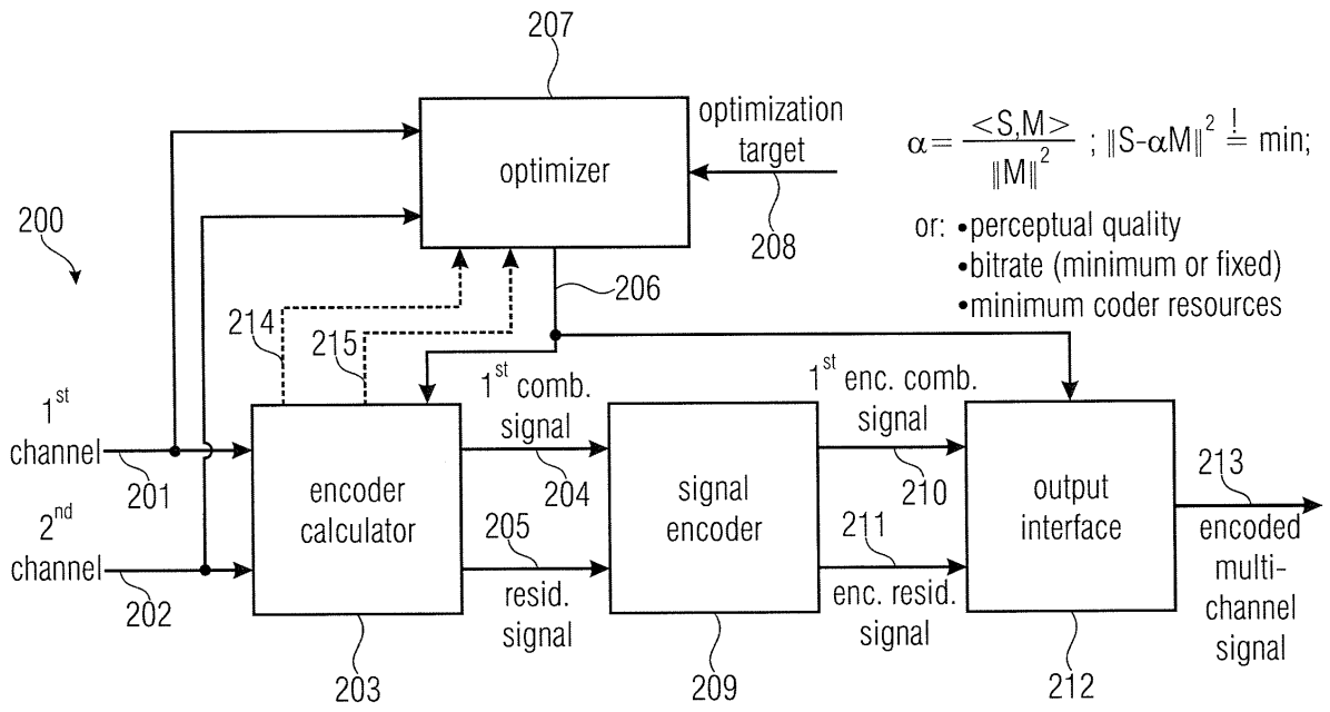
FIGURE 2 (AUDIO ENCODER)
