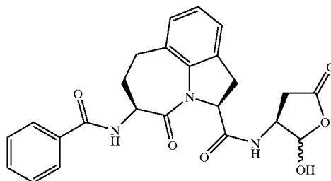
(2S-cis)-[5-Benzoylamino-1,2,3,4,5,6,7-hexahydro-4-oxoazepino[3,2,1-hi]indole-2-carbonyl)-amino]-4-oxo-butanoic Acid
