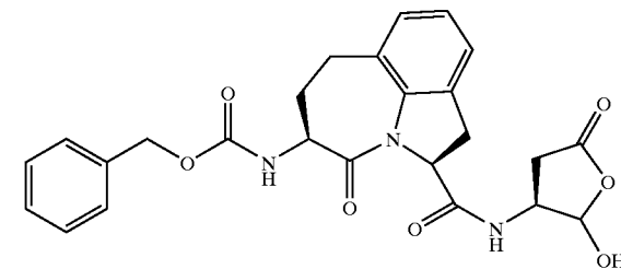
(2S-cis)-5-[Benzyloxycarbonylamino-1,2,4,5,6,7-hexahydro-4-oxazepino[3,2,1-hi]indole-2-carbonyl)-amino]-4-oxo-butanoic Acid
