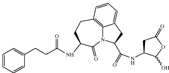
(2S-cis)-[5-Dihydrocinnamylamino-1,2,3,4,5,6,7-hexahydro-4-oxoazepino[3,2,1-hi]indole-2-carbonyl)-amino]-4-oxo-butanoic Acid
