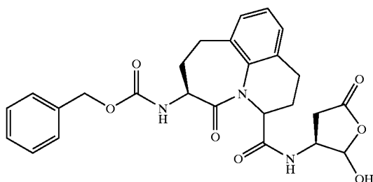
(3R,S-cis)-6-Benzyloxycarbonylamino-5-oxo-2,3,4,5,6,7,8-hexahydro-1H-azepino[3,2,1-hi]quinoline-3-carbonyl-amino]-4-oxo-butanoic Acid
