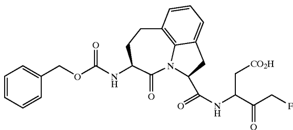
3{(2S-cis)-[5-Benzyloxycarbonylamino-1,2,3,4,5,6,7-hexahydro-4-oxoazepino[3,2,1-hi]indole-2-carbonyl]-amino}-5-fluoro-4-oxo-pentanoic Acid
