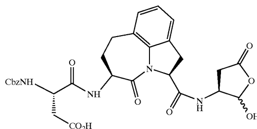
(2S-cis)-[5-(N-Benzyloxycarbonyl-(S)-aspartyl)amino-1,2,3,4,5,6,7-hexahydro-4-oxoazepino[3,2,1-hi]indole-2-carbonyl)-amino]-4-oxo-butanoic Acid
