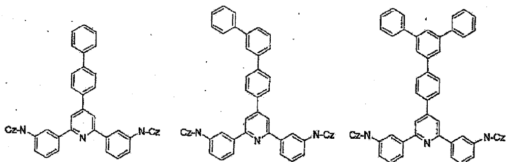
[Chem 11]
