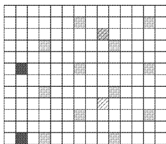
CELL 1 CELL 2 SPECIFIC DM-RS CSI-RS DATA PUNCTURING ADDITIONAL DM-RS FOR MEASURING POWER
