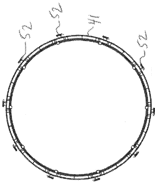
Top View FIG. 7A
