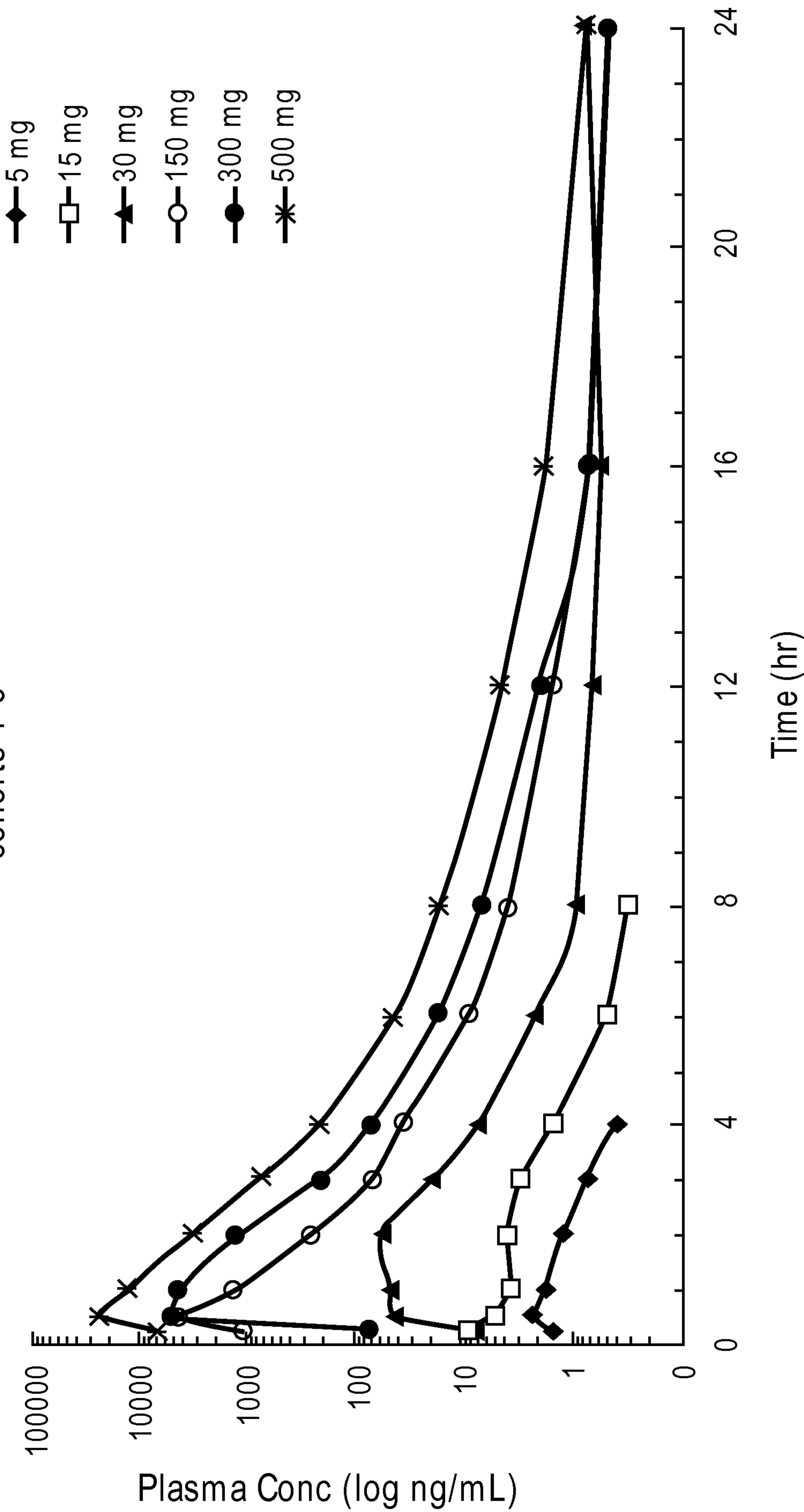
FIG. 8 Plasma concentrations profiles for Compound 1, Na Salt SAD cohorts 1-6
