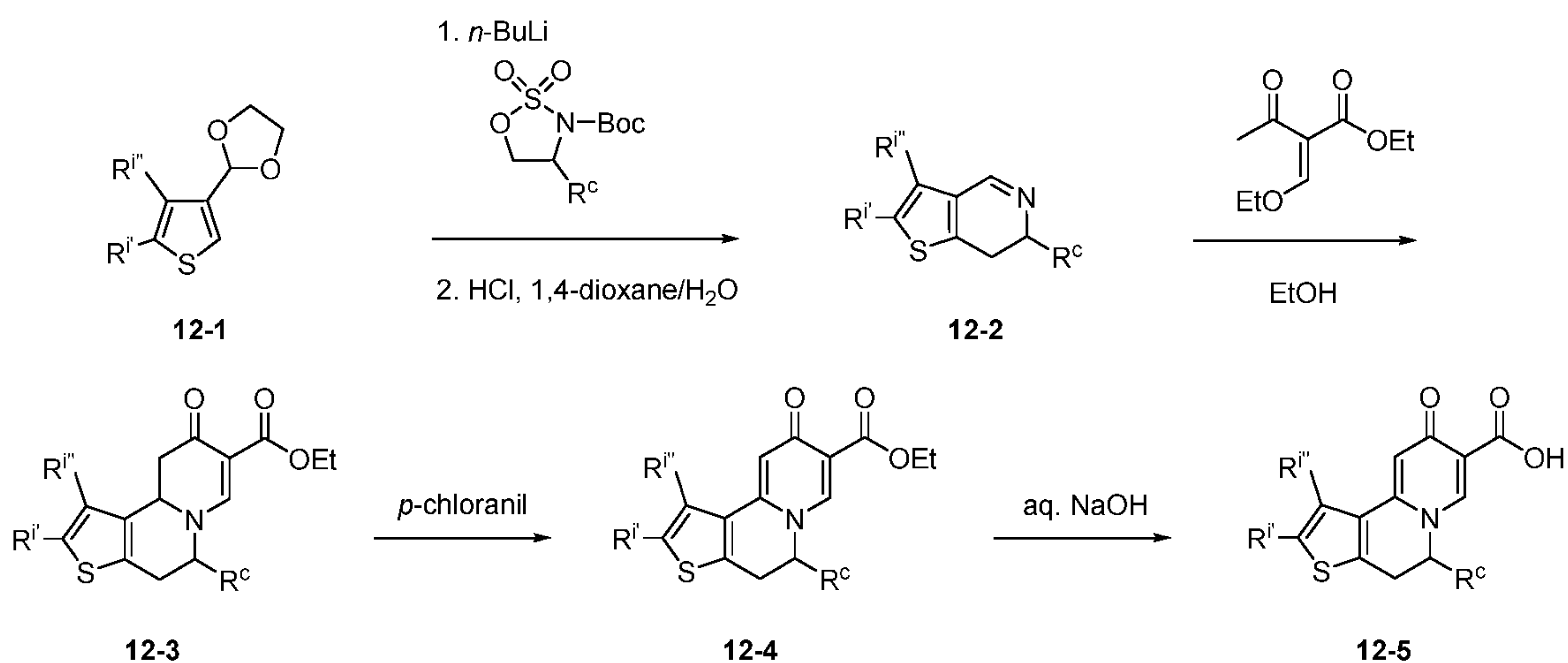
Scheme XII.
