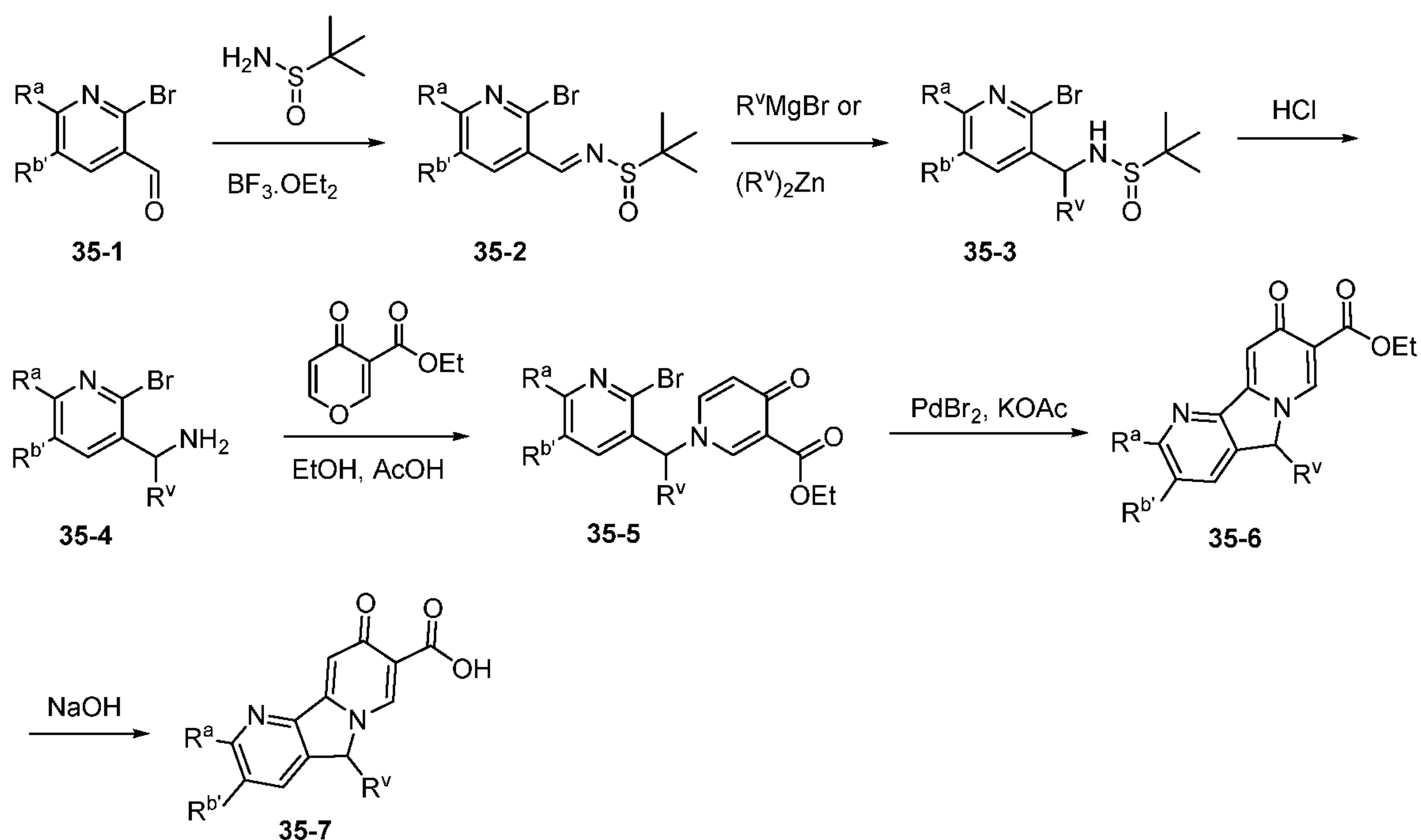
Scheme XXXV.
