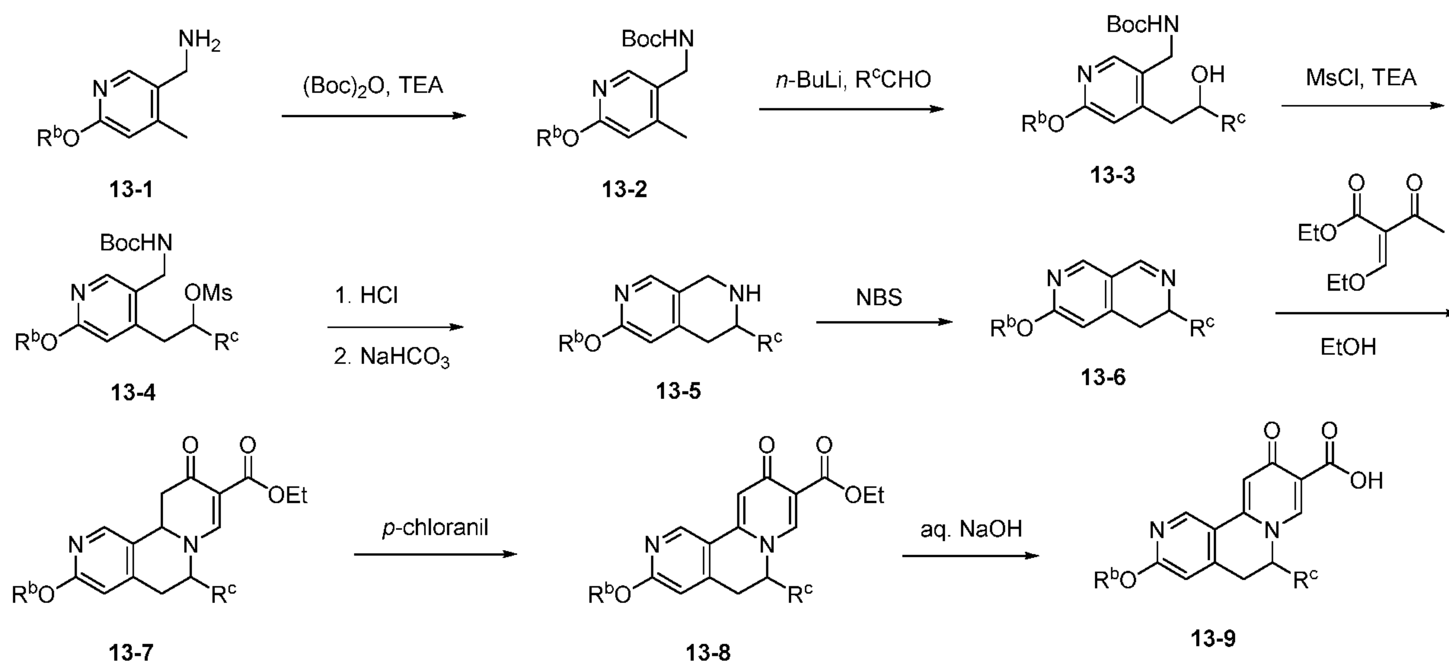
Scheme XIII.
