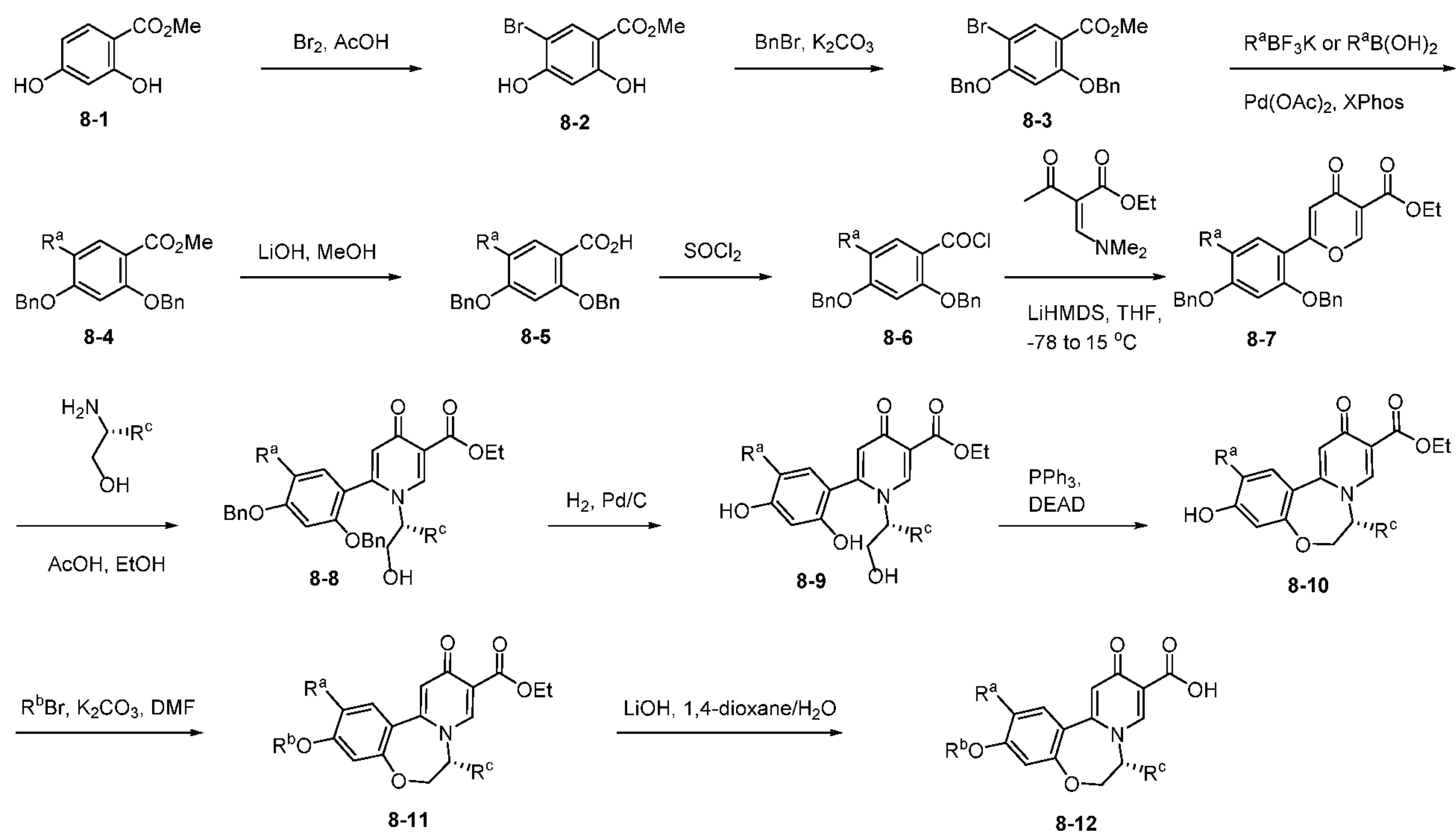
Scheme VIII.
