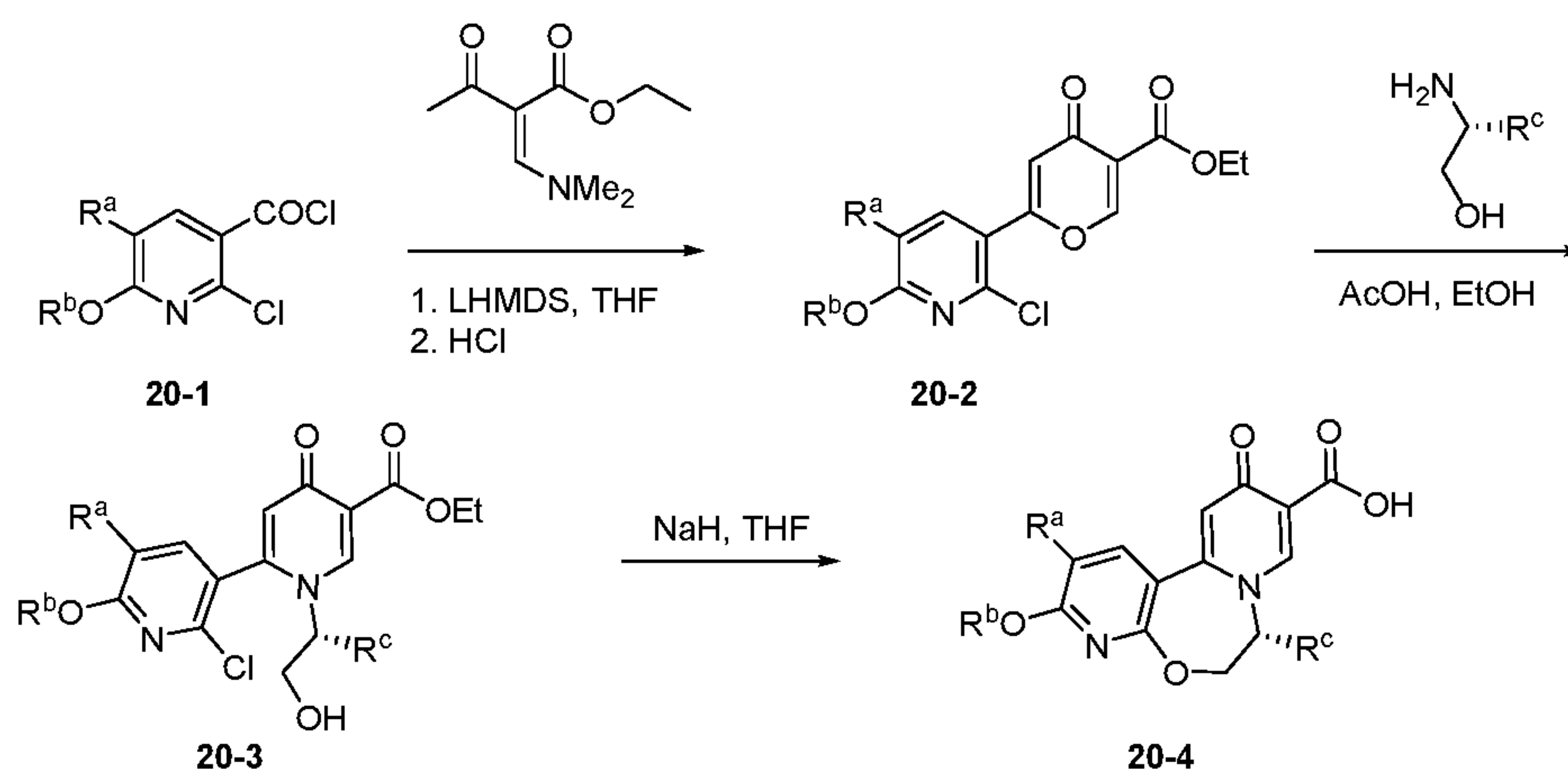
Scheme XX.
