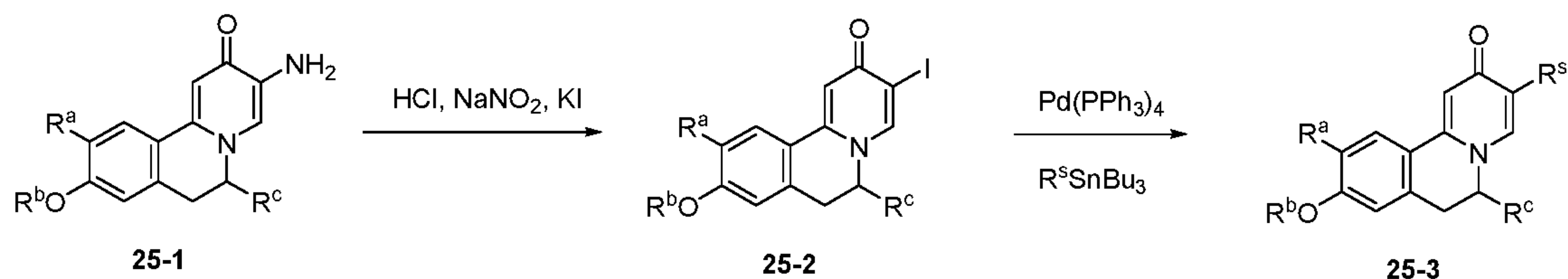
Scheme XXV.
