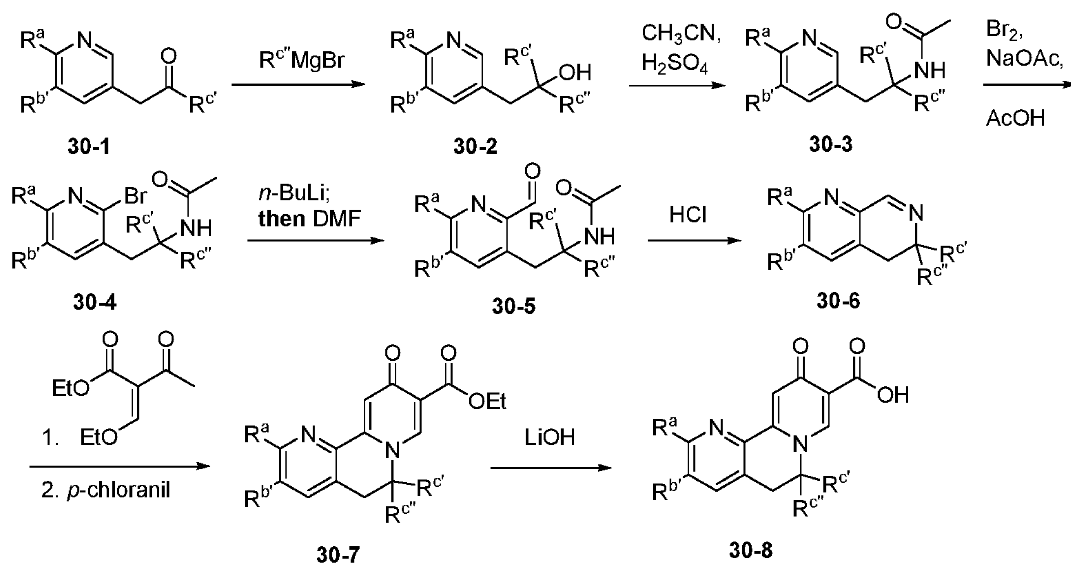
Scheme XXX.
