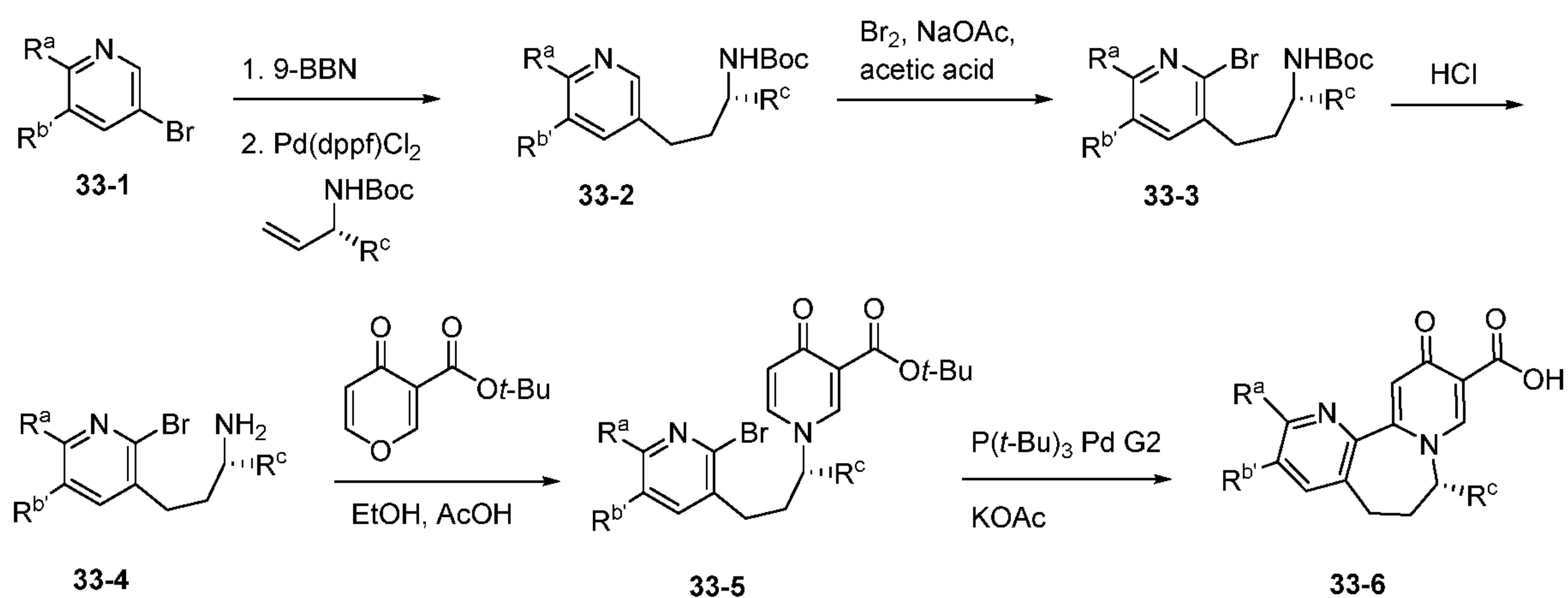
Scheme XXXIII.
