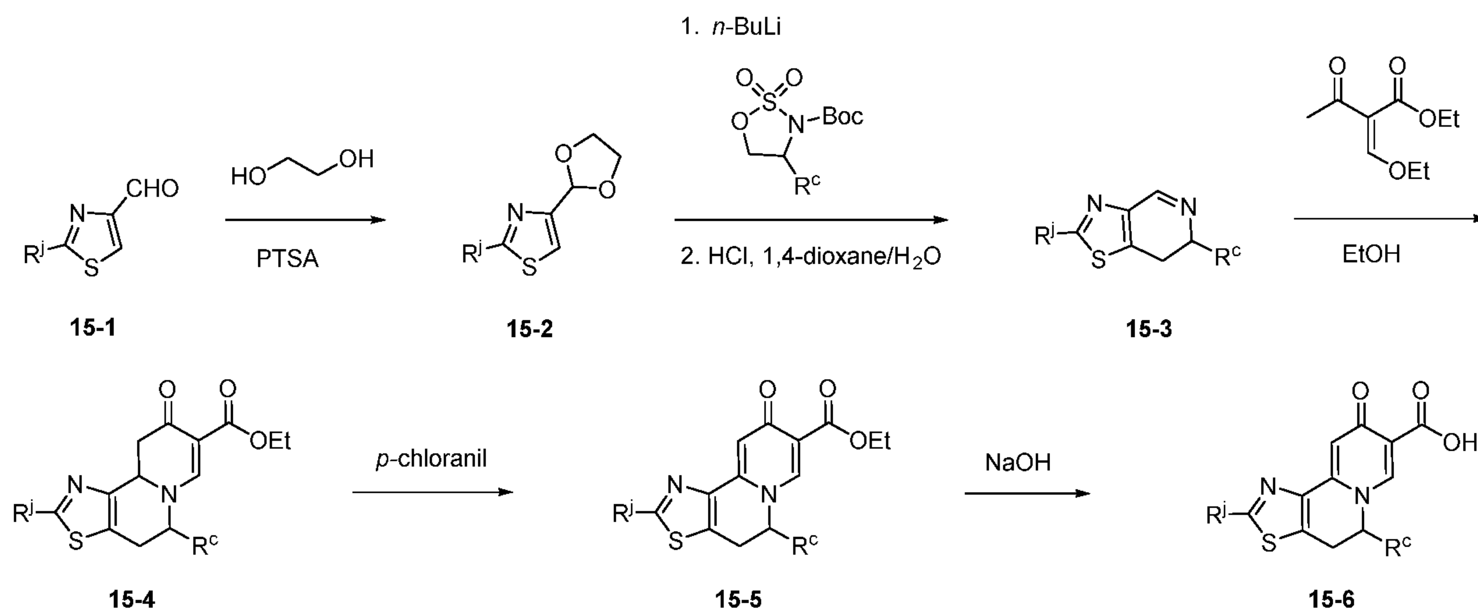
Scheme XV.
