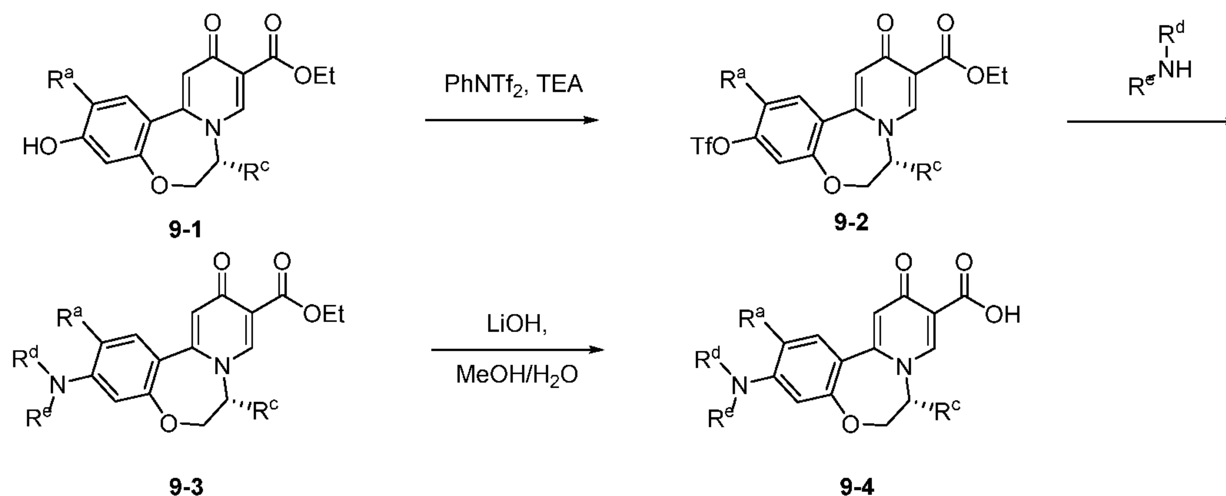
Scheme IX.
