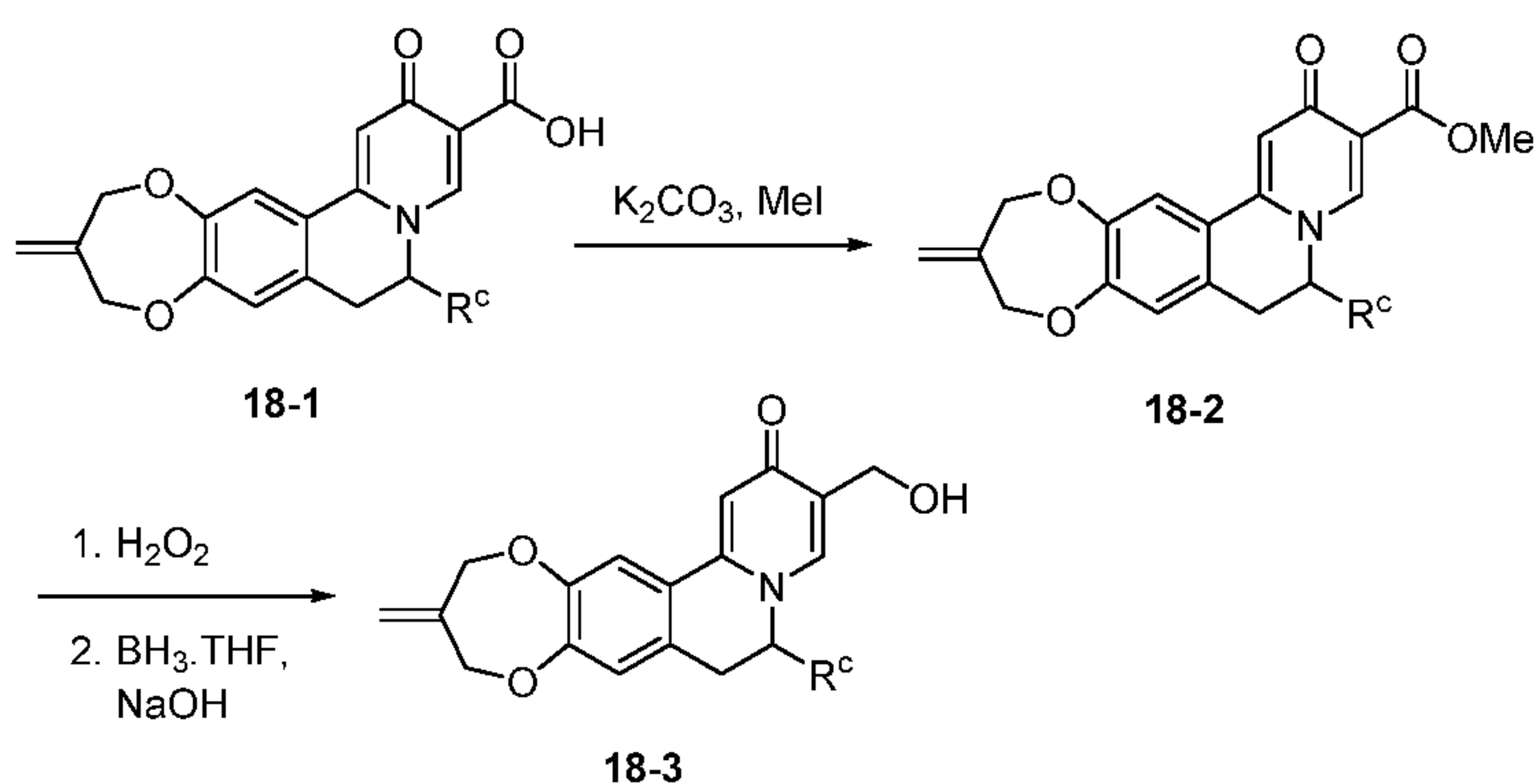
Scheme XVIII.
