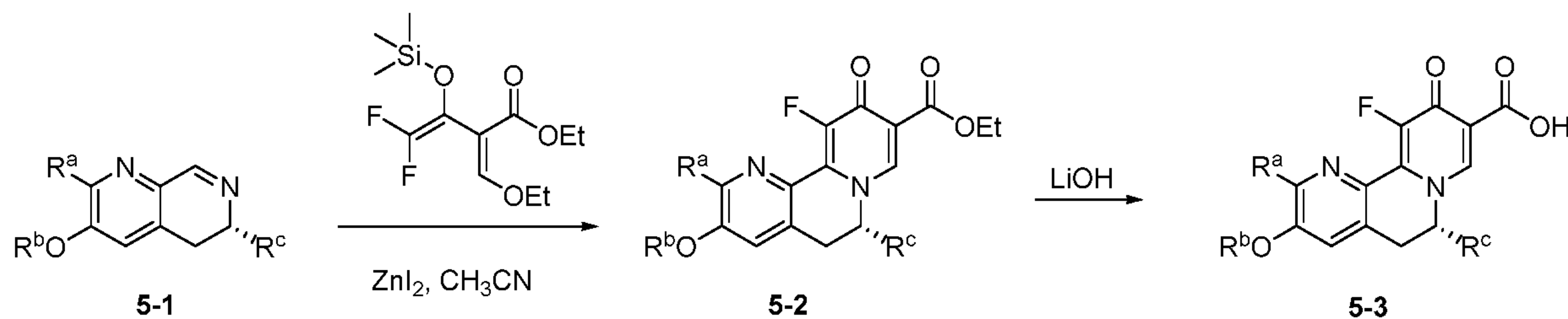
Scheme V.
