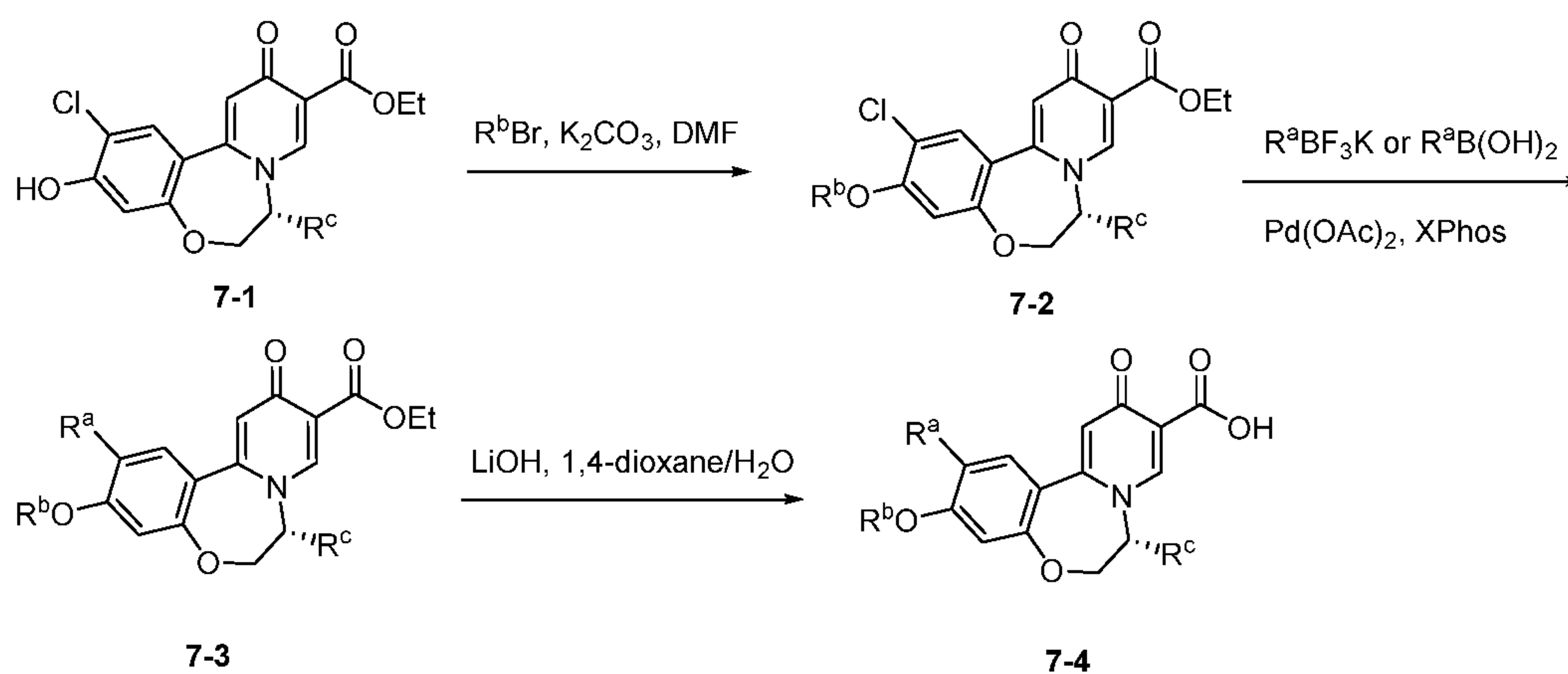
Scheme VII.
