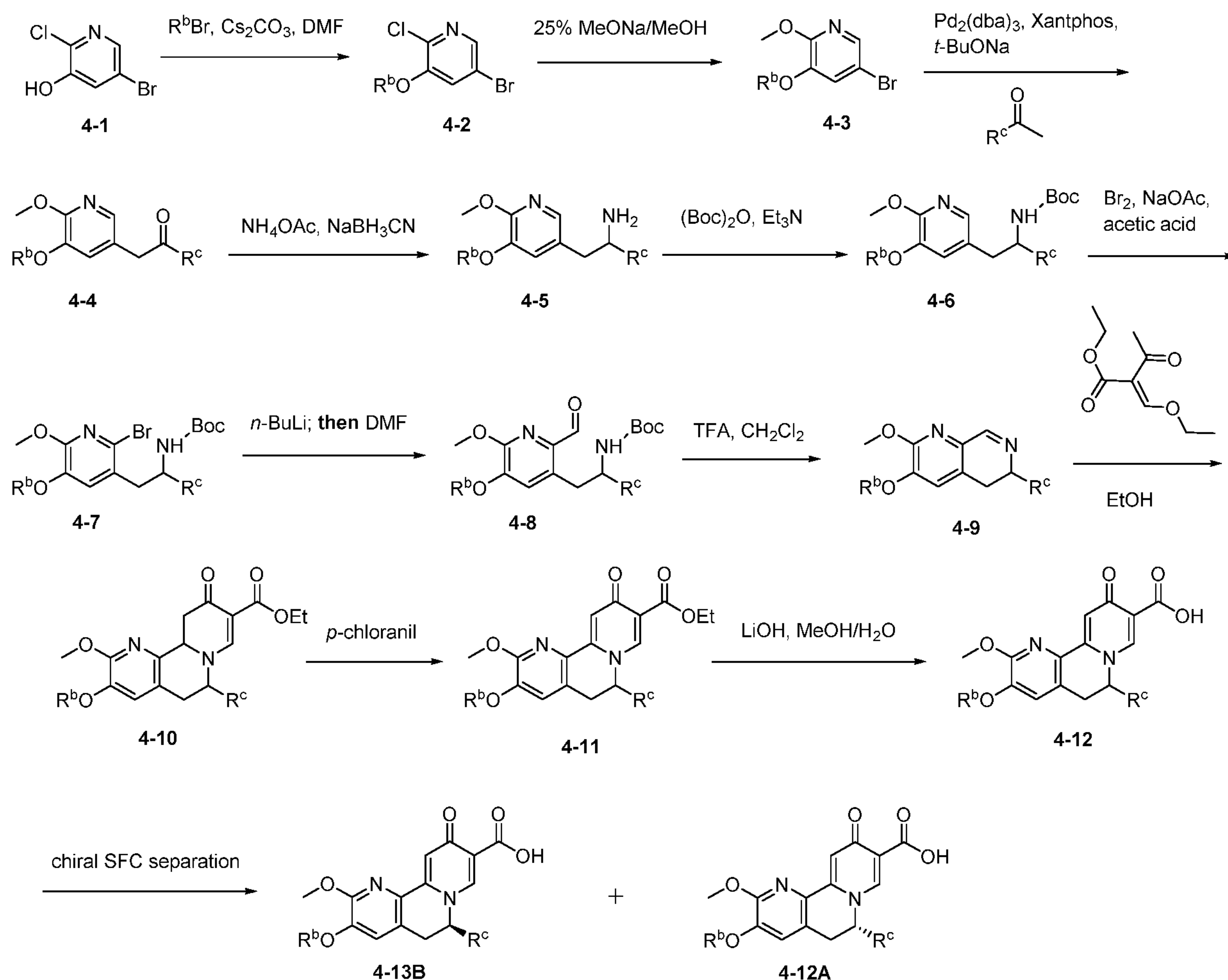
Scheme IV.
