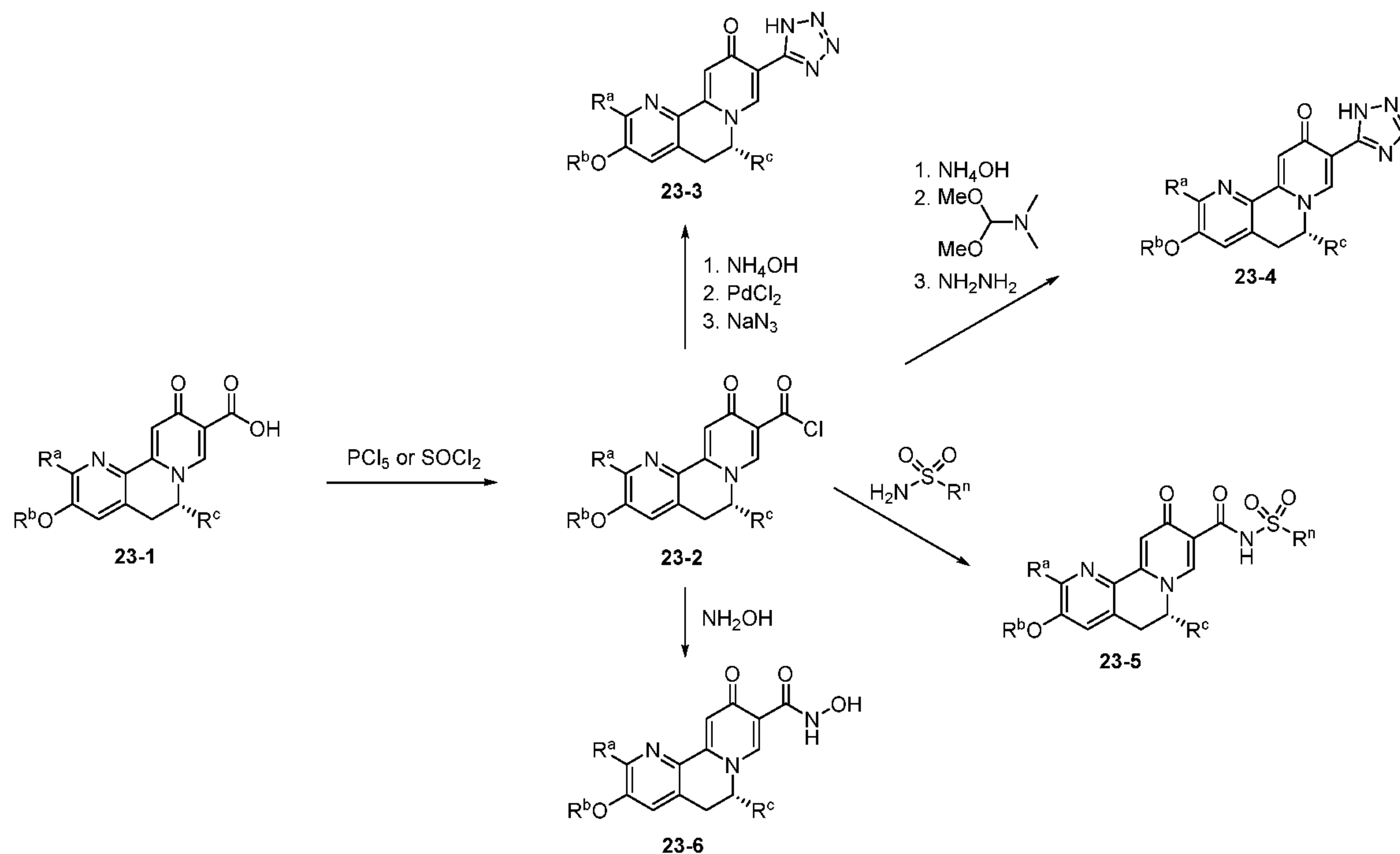
Scheme XXIII.
