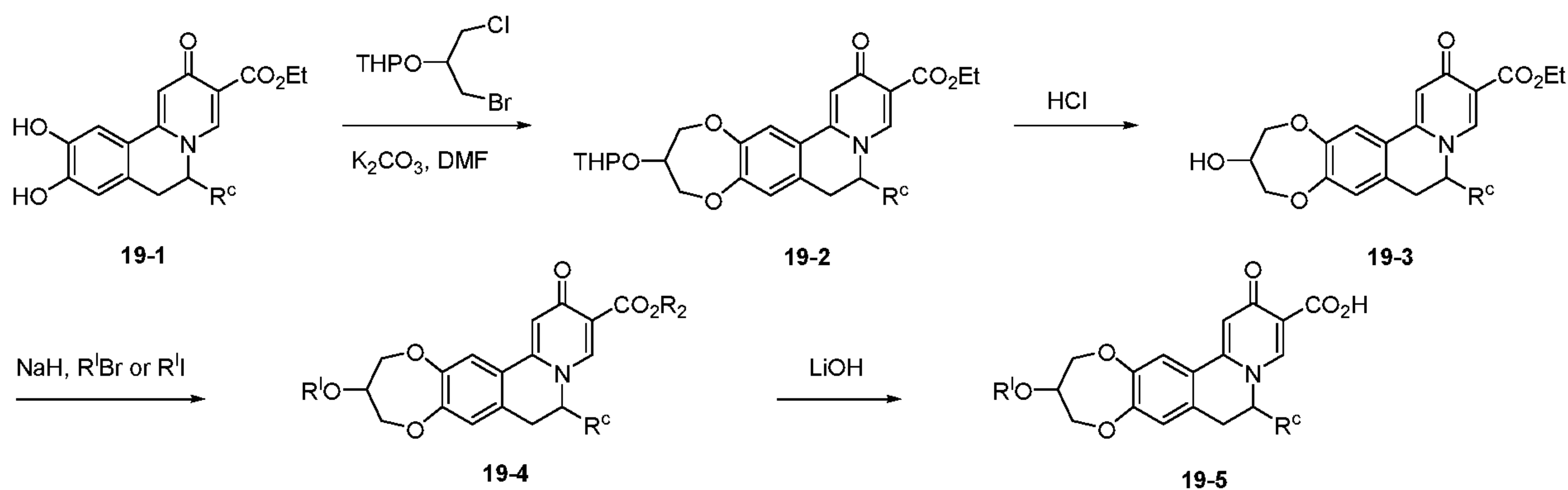
Scheme XIX.
