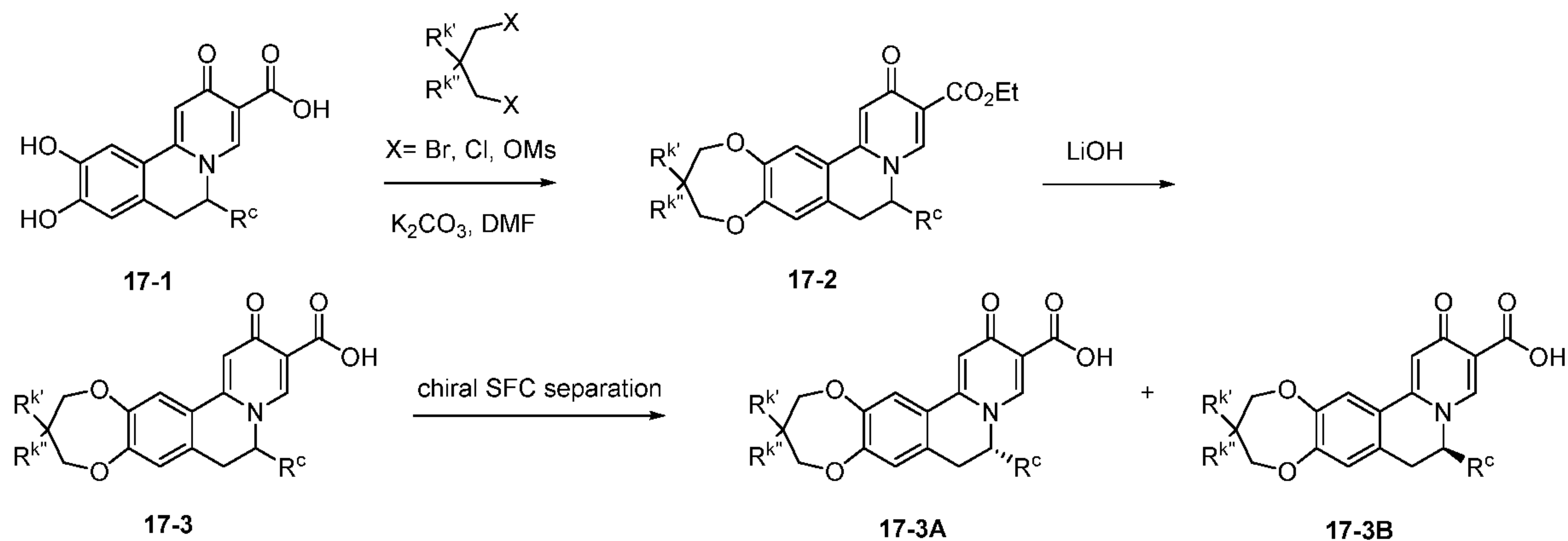
Scheme XVII.
