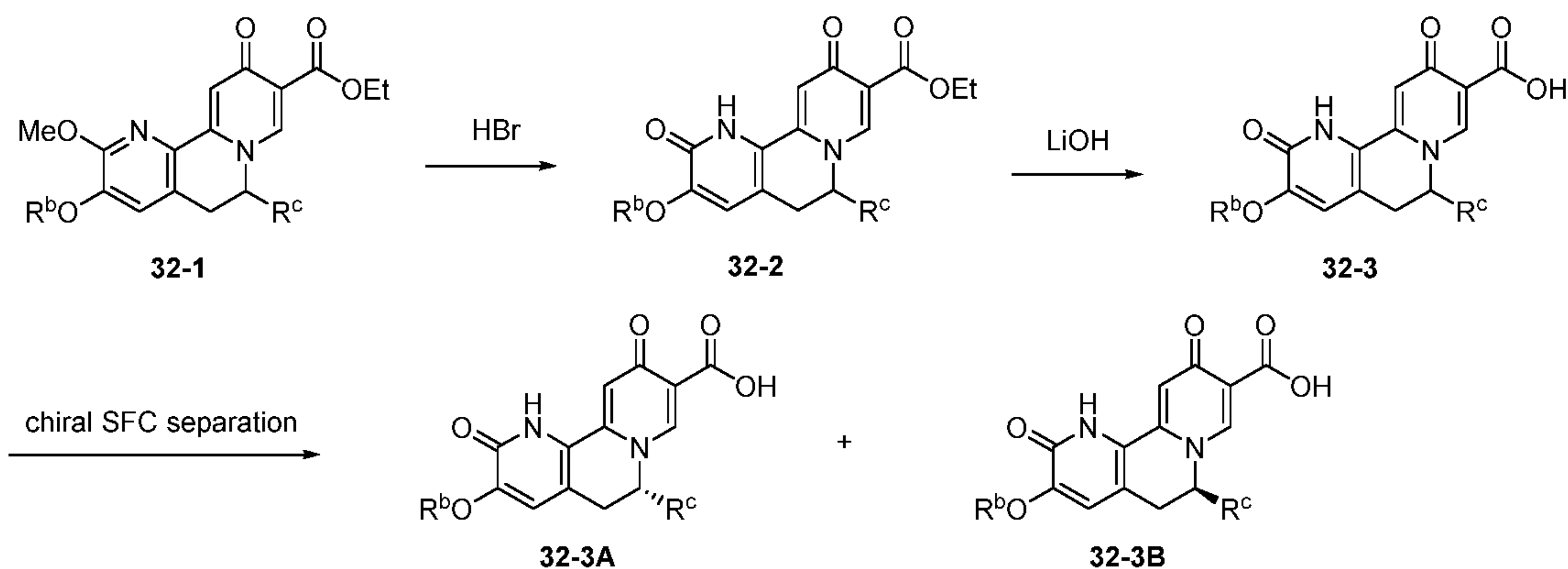
Scheme XXXII.
