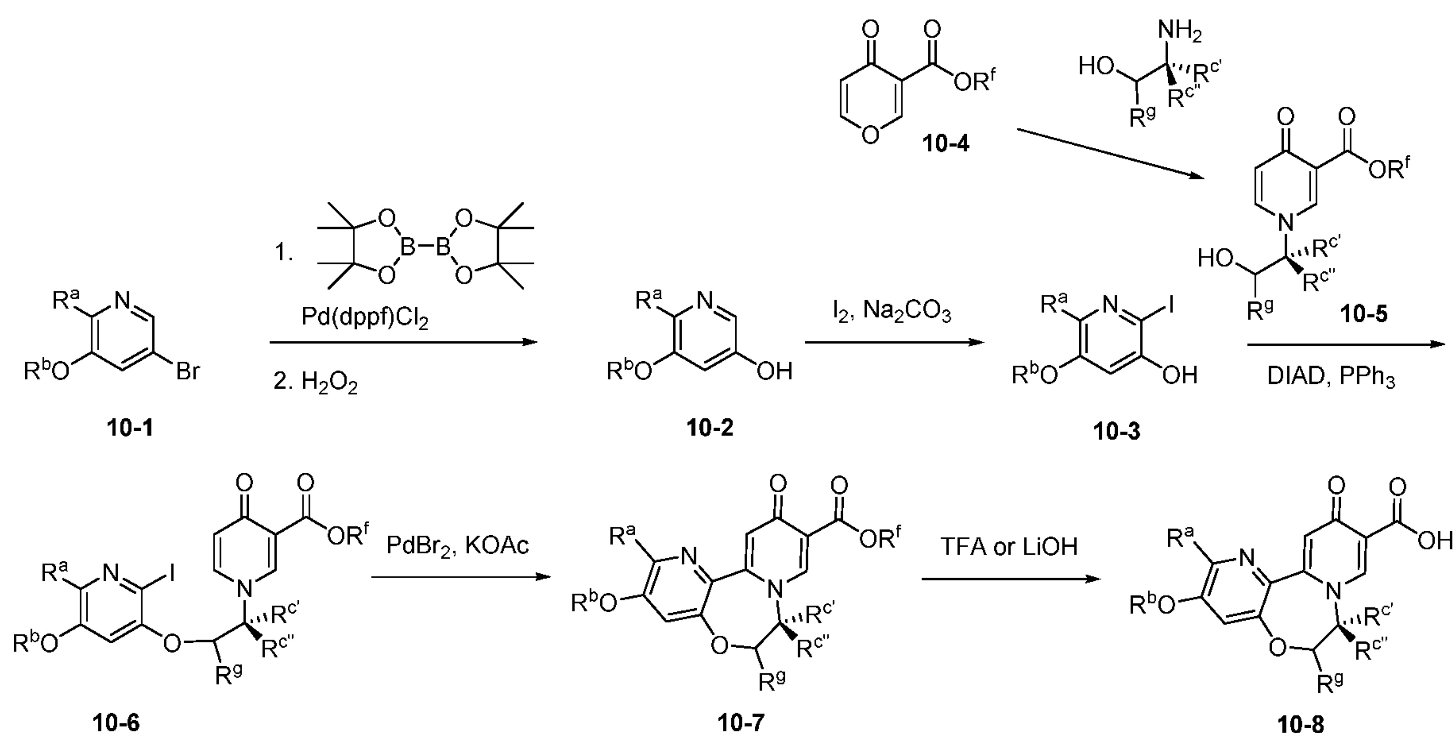
Scheme X.
