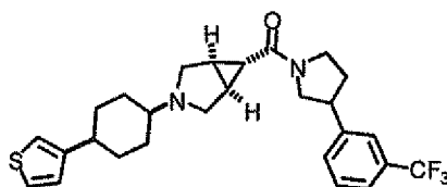
Intermediate 5f
