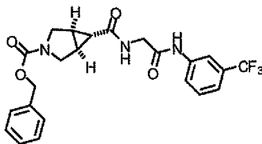
Intermediate 4d
