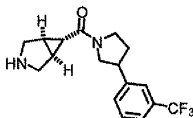
Intermediate 5b
