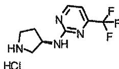
Intermediate 6b
