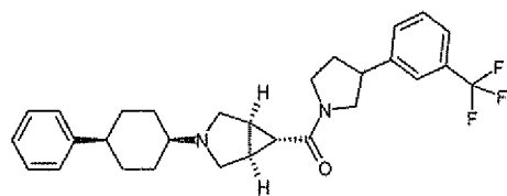
Diastereomer A
