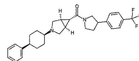
Diastereomer B
