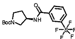
Intermediate-7a
