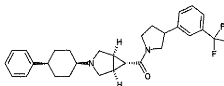
Diastereomer B
