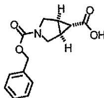
Intermediate 4c
