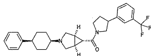
Diastereomer C
