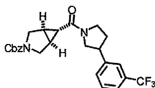
Intermediate 5a
