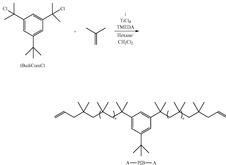
Scheme 1 Strategy for the Synthesis of HO-S-PIB-S-OH
