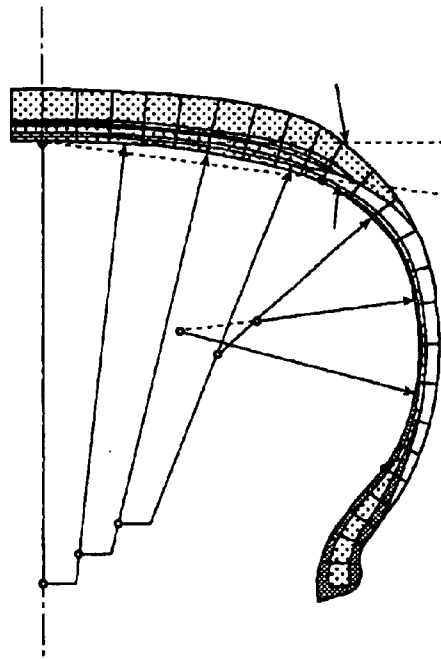
FIG. 9B PRIOR ART
