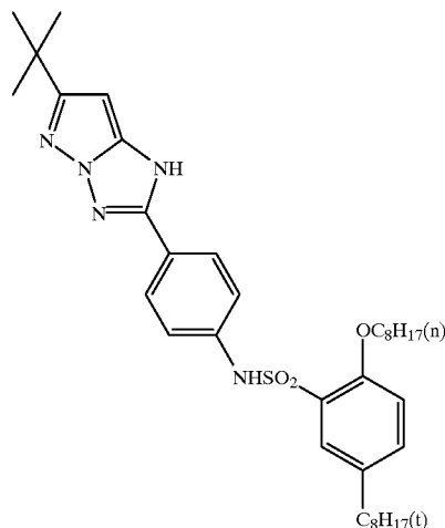
Magenta dye forming coupler (a1)
