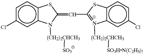
sensitizing dye I for blue-sensitive emulsions
