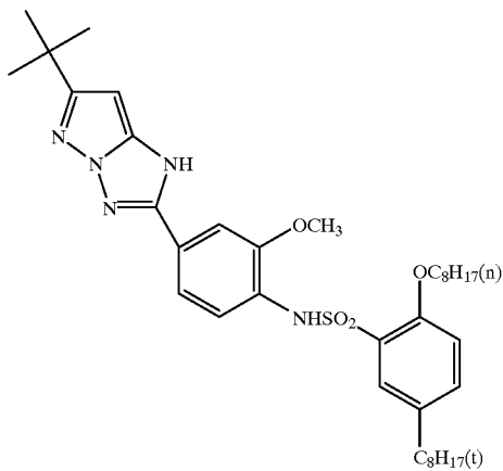
Magenta coupler (a1) magenta coupler (coupler of the present invention)
