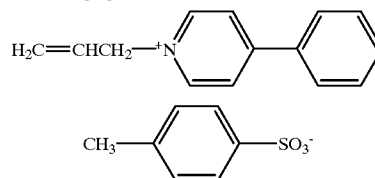
crystal habit controlling agent 4
