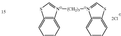
crystal habit controlling agent 30
