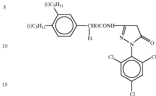
Magenta coupler (a1) magenta coupler (coupler of the present invention)
