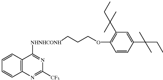
Developing agent (v)
