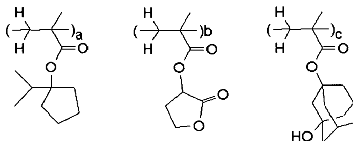
Polymer 4 (a=0.50, b=0.40, c=0.10, Mw=7,700)
