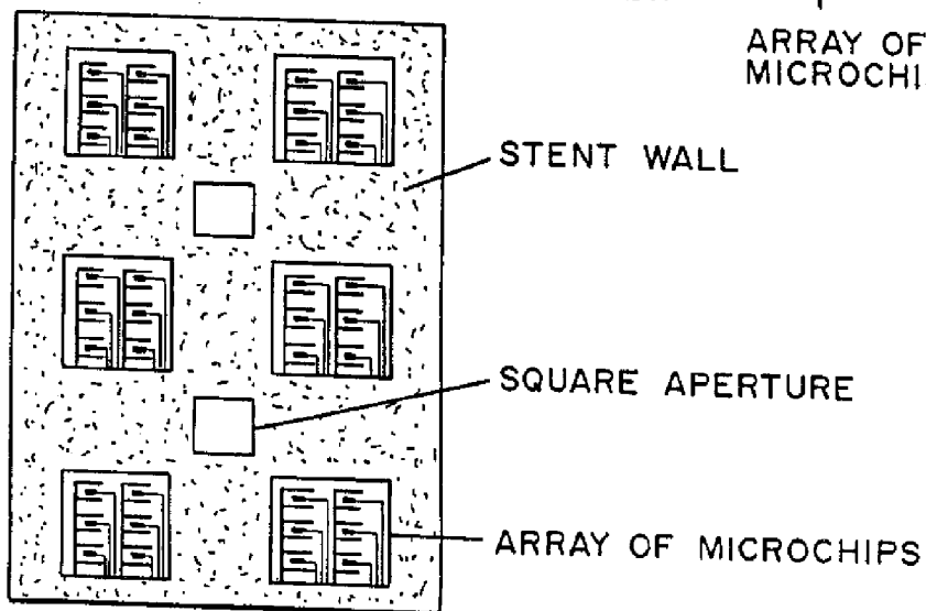
FIG. 9B VERTICAL CROSS-SECTIONAL VIEW
