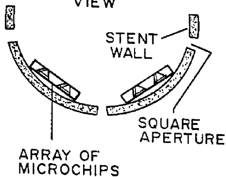
FIG. 9C VERTICAL CROSS-SECTIONAL VIEW
