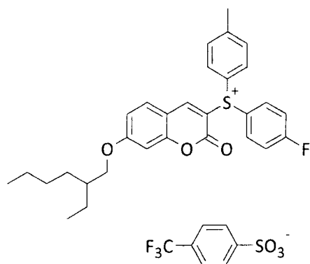
Compound No. 10
