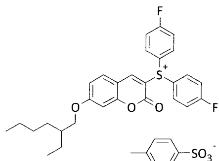
Compound No. 8
