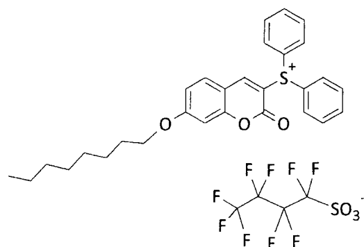
Compound No. 16
