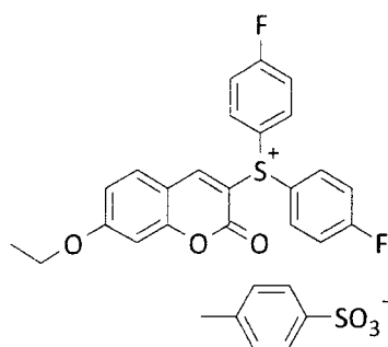
Compound No. 1
