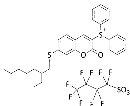
Compound No. 42
