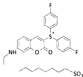
Compound No. 34
