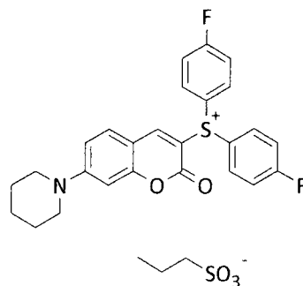
Compound No. 32
