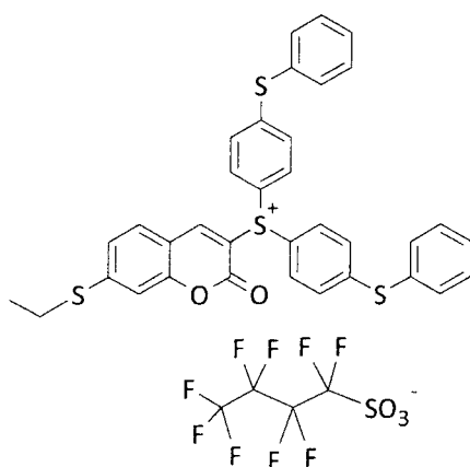
Compound No. 47
