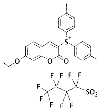
Compound No. 20
