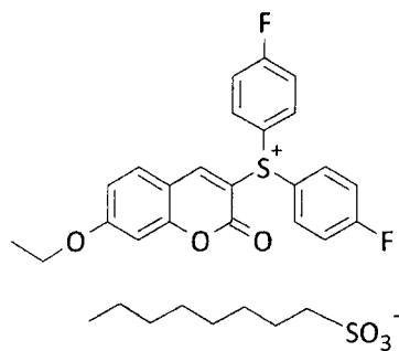
Compound No. 6
