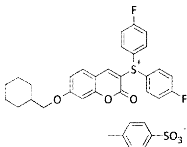
Compound No. 19
