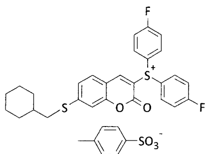
Compound No. 43
