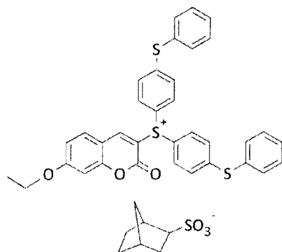
Compound No. 23
