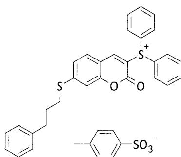
Compound No. 41
