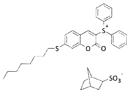
Compound No. 39
