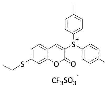
Compound No. 44
