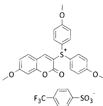
Compound No. 25
