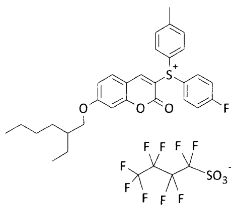
Compound No. 9
