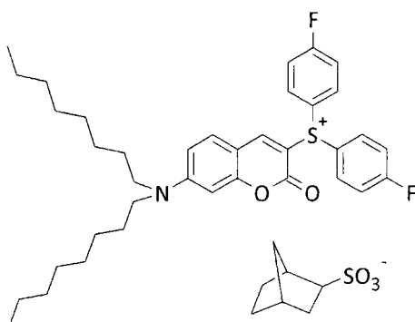
Compound No. 31
