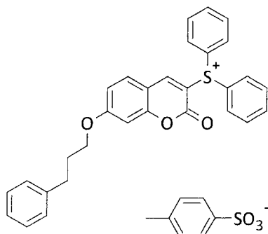
Compound No. 15
