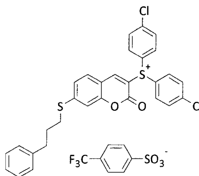
Compound No. 46
