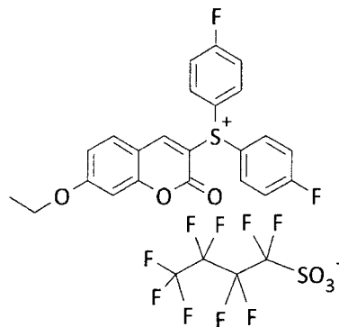
Compound No. 2
