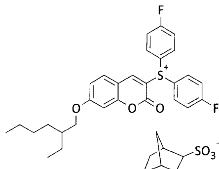
Compound No. 12
