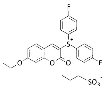
Compound No. 7
