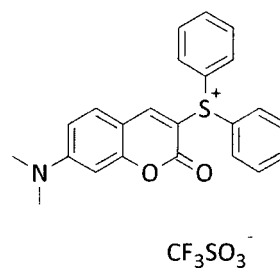
Compound No. 30
