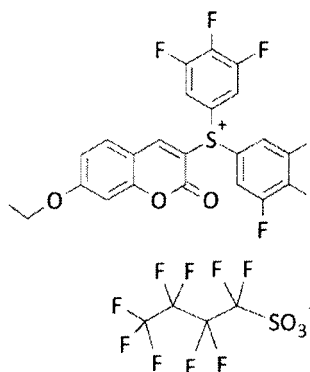
Compound No. 24
