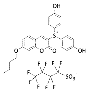
Compound No. 36
