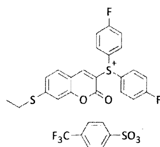
Compound No. 38
