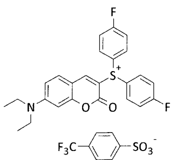
Compound No. 29
