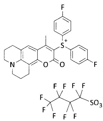
Compound No. 48
