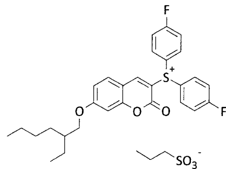
Compound No. 14
