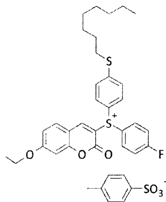
Compound No. 17
