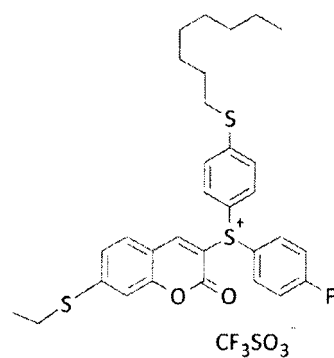
Compound No. 40
