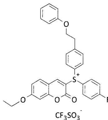
Compound No. 26
