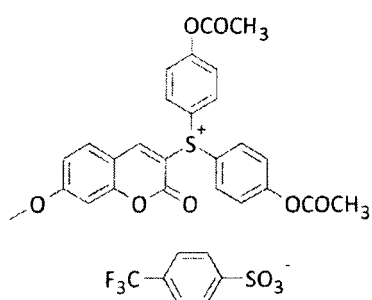
Compound No. 37
