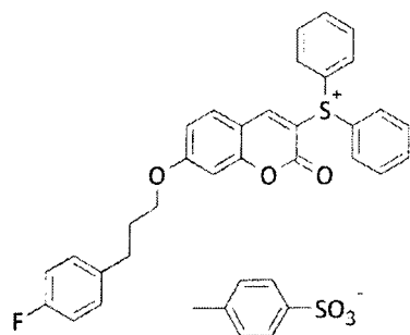
Compound No. 35
