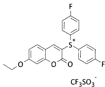
Compound No. 4
