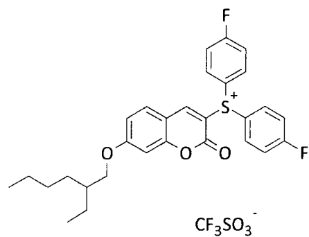
Compound No. 11
