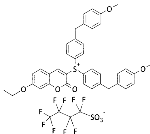
Compound No. 28
