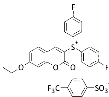
Compound No. 3
