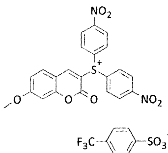
Compound No. 21
