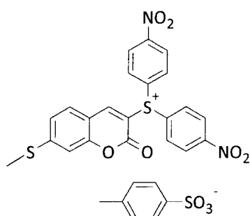
Compound No. 45
