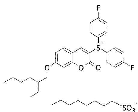
Compound No. 13
