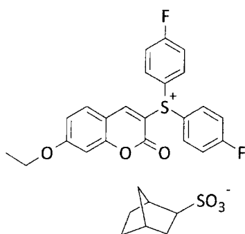
Compound No. 5
