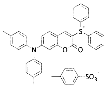
Compound No. 33
