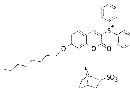
Compound No. 18
