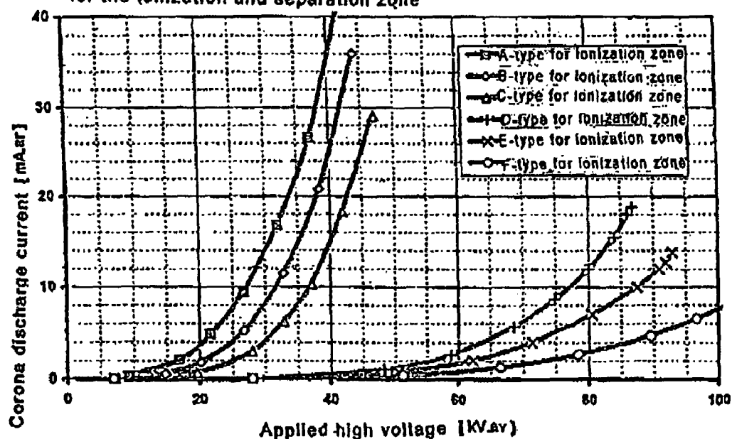
Fig. 2 Examples of individual characteristics of negative electrode forms for the ionization and separation zone
