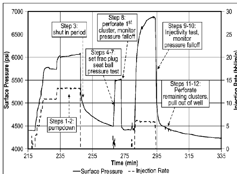
FIG. 3 Pump-down diagnostics and establishing selective injectivity into the first perforation cluster
