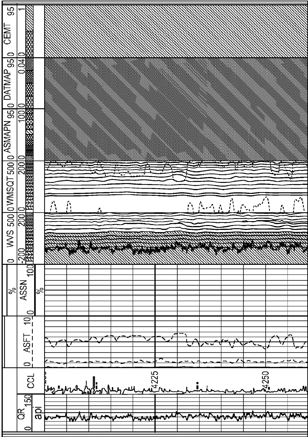
FIG. 18 Cement coverage as measured by Radial Bond Tool, in lateral section covered by fracturing stages 4-5
