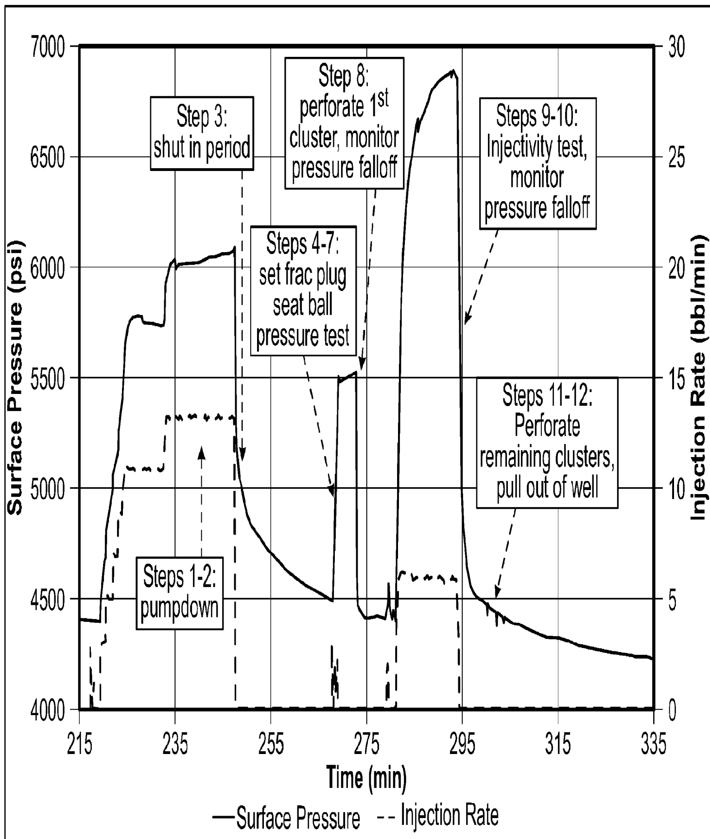
FIG. 3 Pump-down diagnostics and establishing selective injectivity into the first perforation cluster
