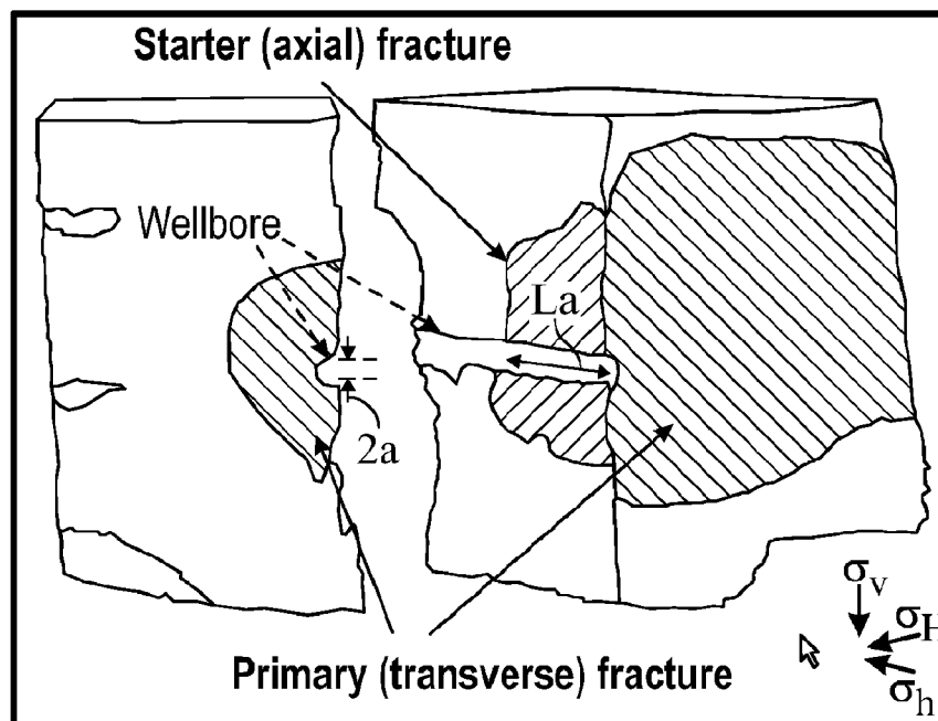
FIG. 2 Longitudinal starter fracture increases the breadth of fracturing along the lateral (Weijers et al 1994)
