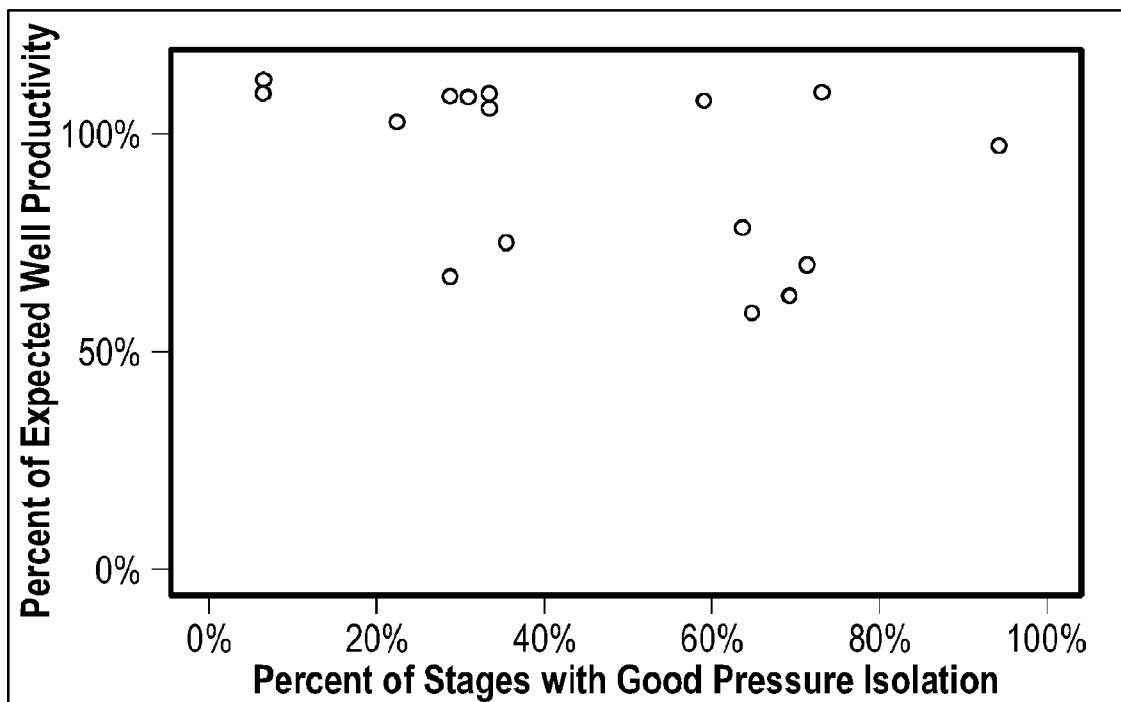
FIG. 25 Scatter plot showing a comparison of well productivity against percent of stages with good pressure isolation. Each point is a well that was completed using 15 ft (4.5 m) cluster spacing.
