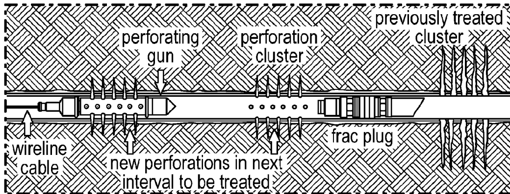
FIG. 1 Plug-and-perf method of simulating multiple intervals in a horizontal well (Stonewall Engineering)
