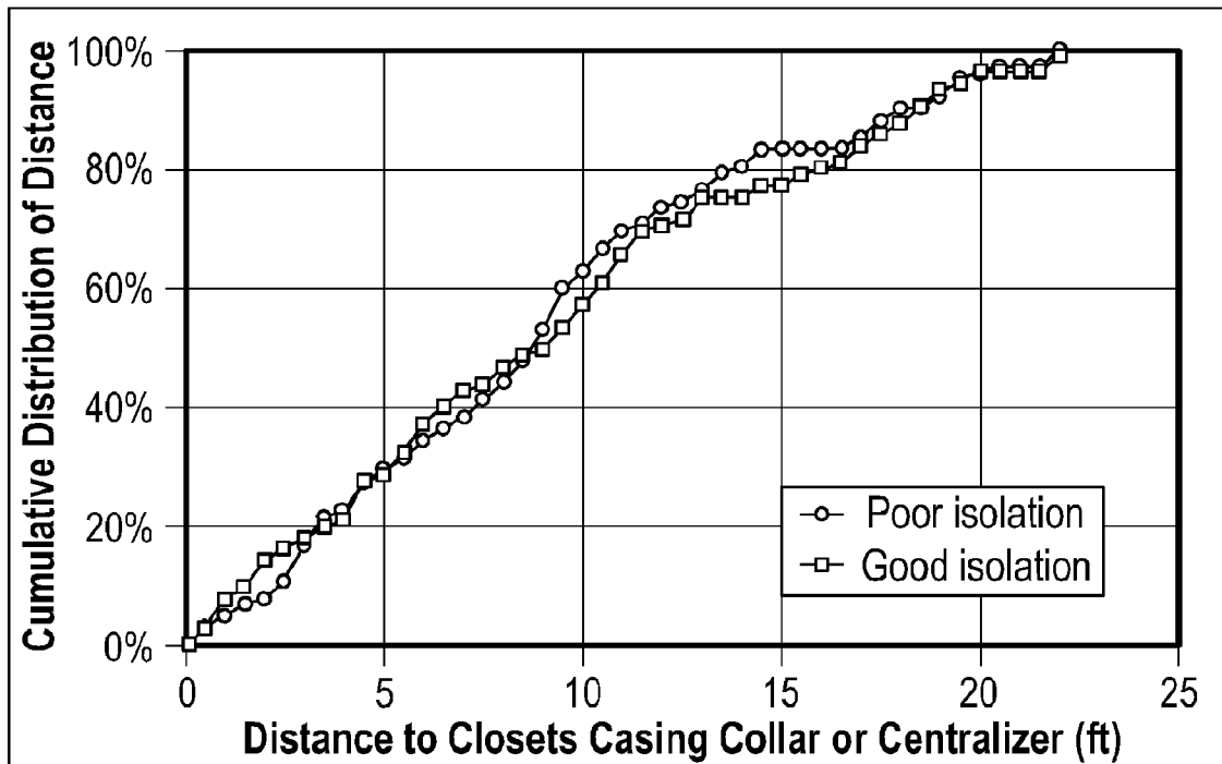
FIG. 24 Cumulative distributions of distance between the 1 st perforation cluster (toe side) and closest casing collar or centralizer location
