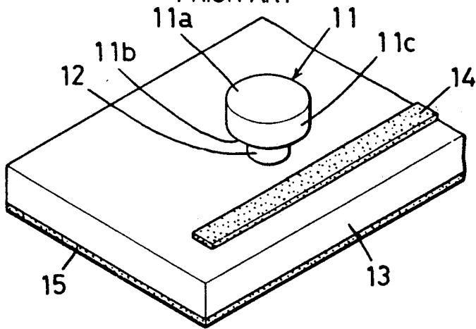
FIG.7 PRIOR ART
