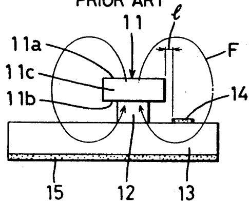
FIG.8 PRIOR ART
