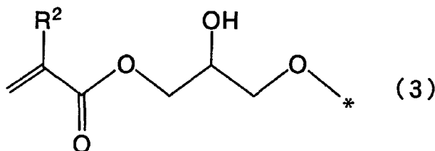
[Chemical Formula 9]
