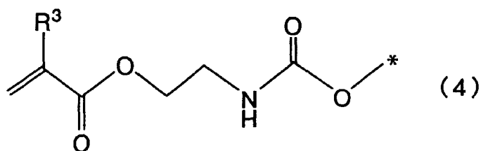
[Chemical Formula 4]
