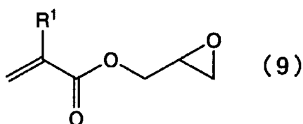
[Chemical Formula 15]
