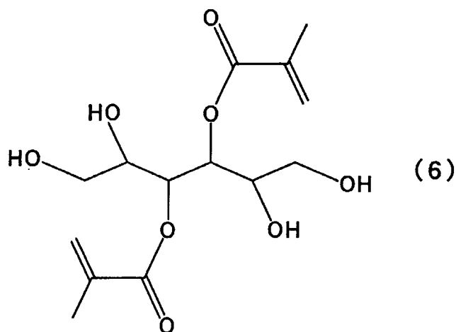
[Chemical Formula 12]
