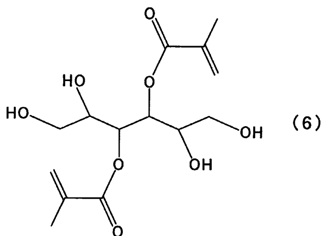
[Chemical Formula 6]
