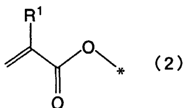
[Chemical Formula 2]
