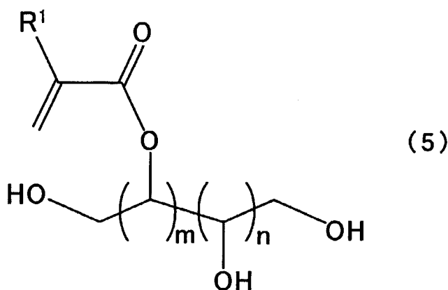
[Chemical Formula 11]
