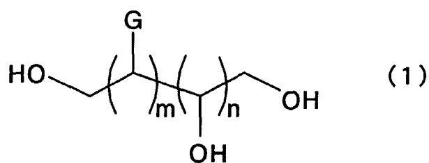
[Chemical Formula 1]
