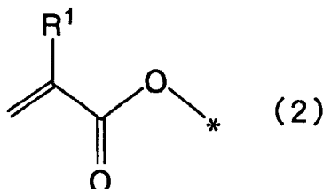
[Chemical Formula 8]
