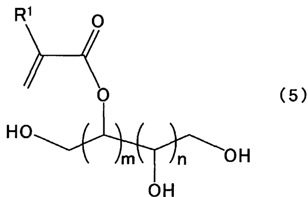
[Chemical Formula 5]
