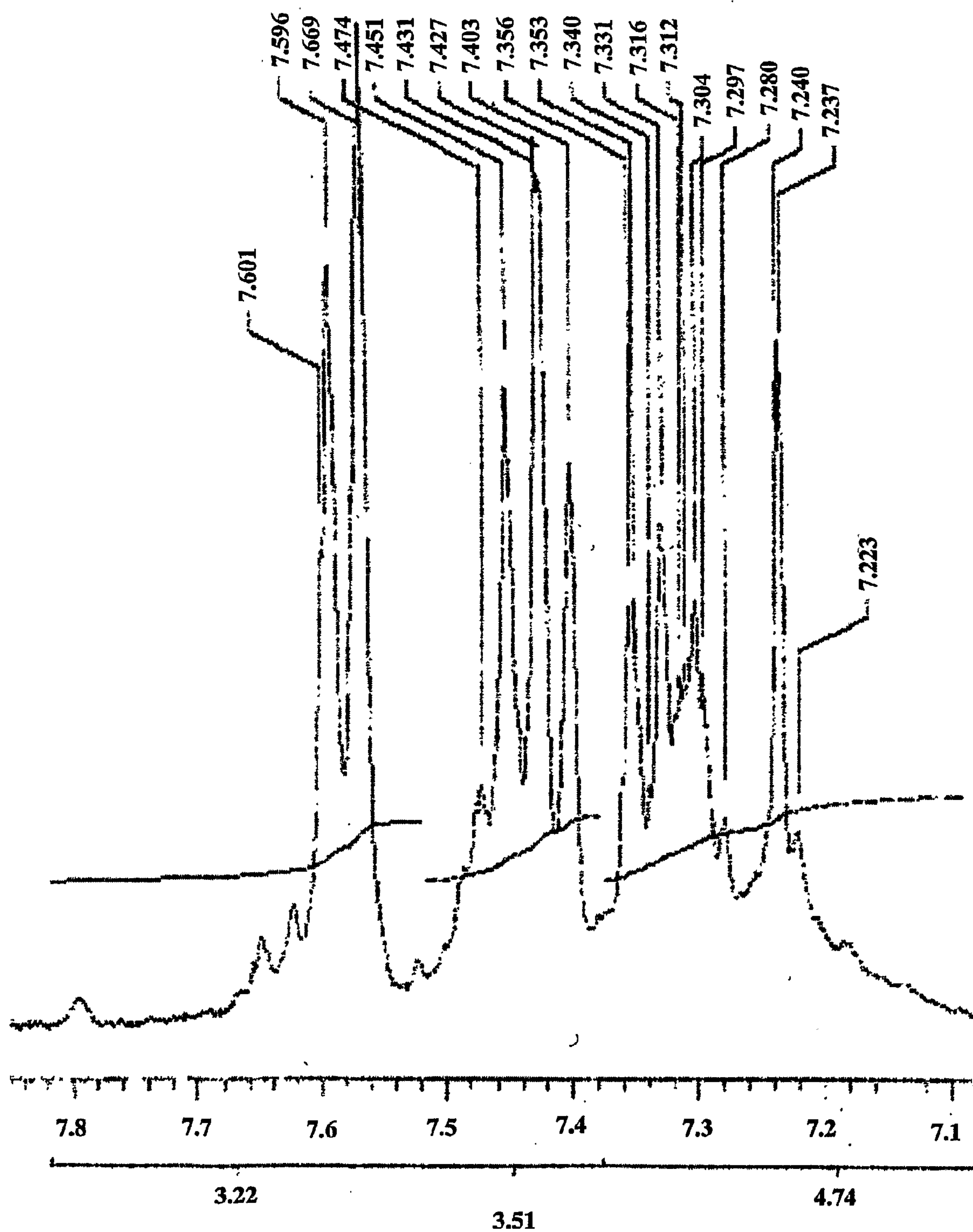
C. ^1\text{H} NMR Spectrum SUBSTITUTE SHEET (RULE 26)
