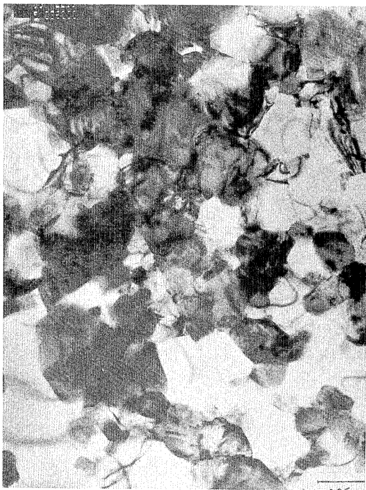
Al - 12 Fe - 2V As - Extruded
