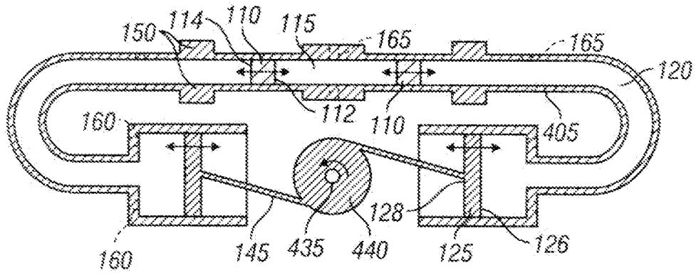
Two-free-Piston , Two Extractor-Piston, Single-Crank Two-Stroke-Embodiment
