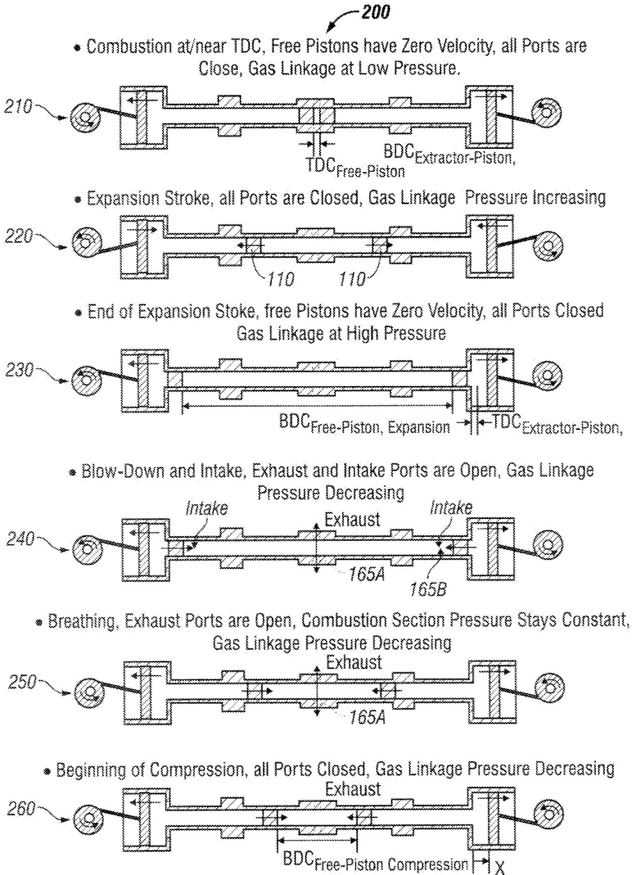
Two Stroke Operation of Two-Free-Piston, Two-Extractor-Piston, Two-Crank Embodiment
