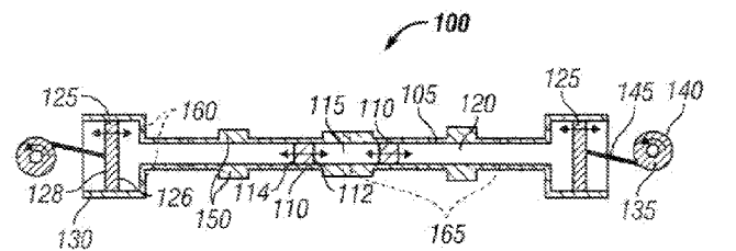
Two-Free-Piston, Two-Extractor-Piston, Two-Crank, Two-Stroke-Embodiment
