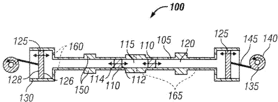
Two-Free-Piston, Two-Extractor-Piston, Two-Crank, Two-Stroke-Embodiment
