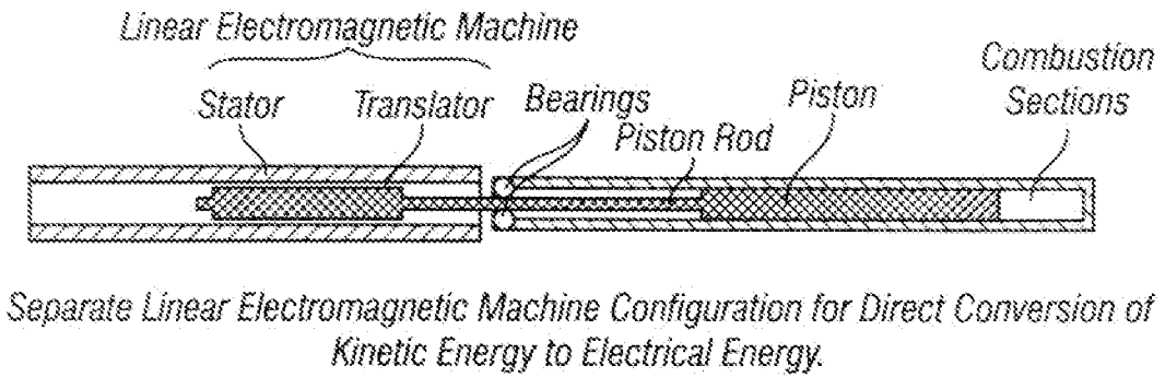
FIG. 4 (Prior Art)
