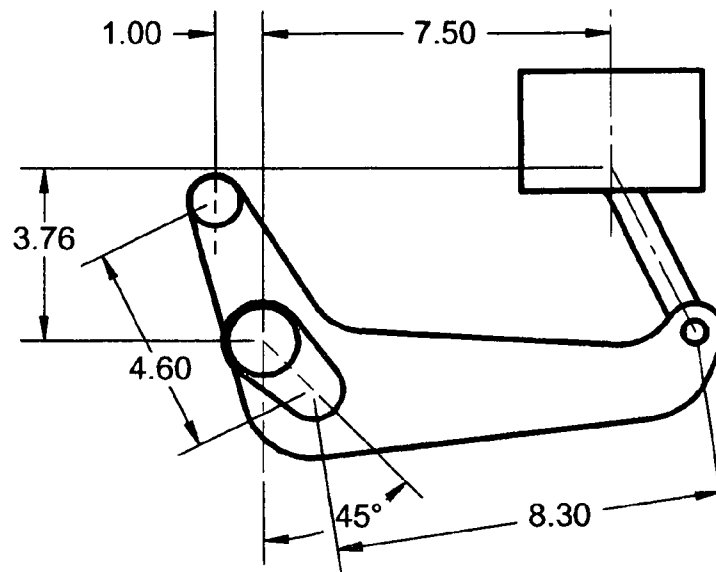
FIG. 5 1" Pathway/Guide Offset
