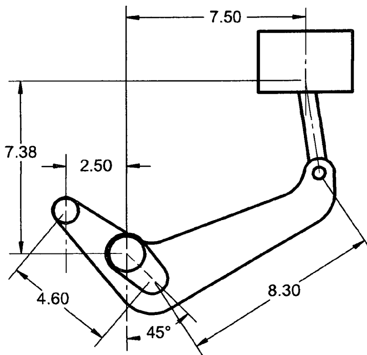
FIG. 6 2.5" Pathway/Guide Offset
