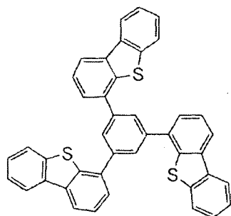
DBT3P-II
