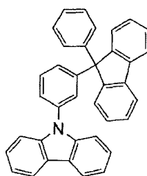
mCzFLP
