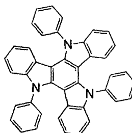
P3Dic
