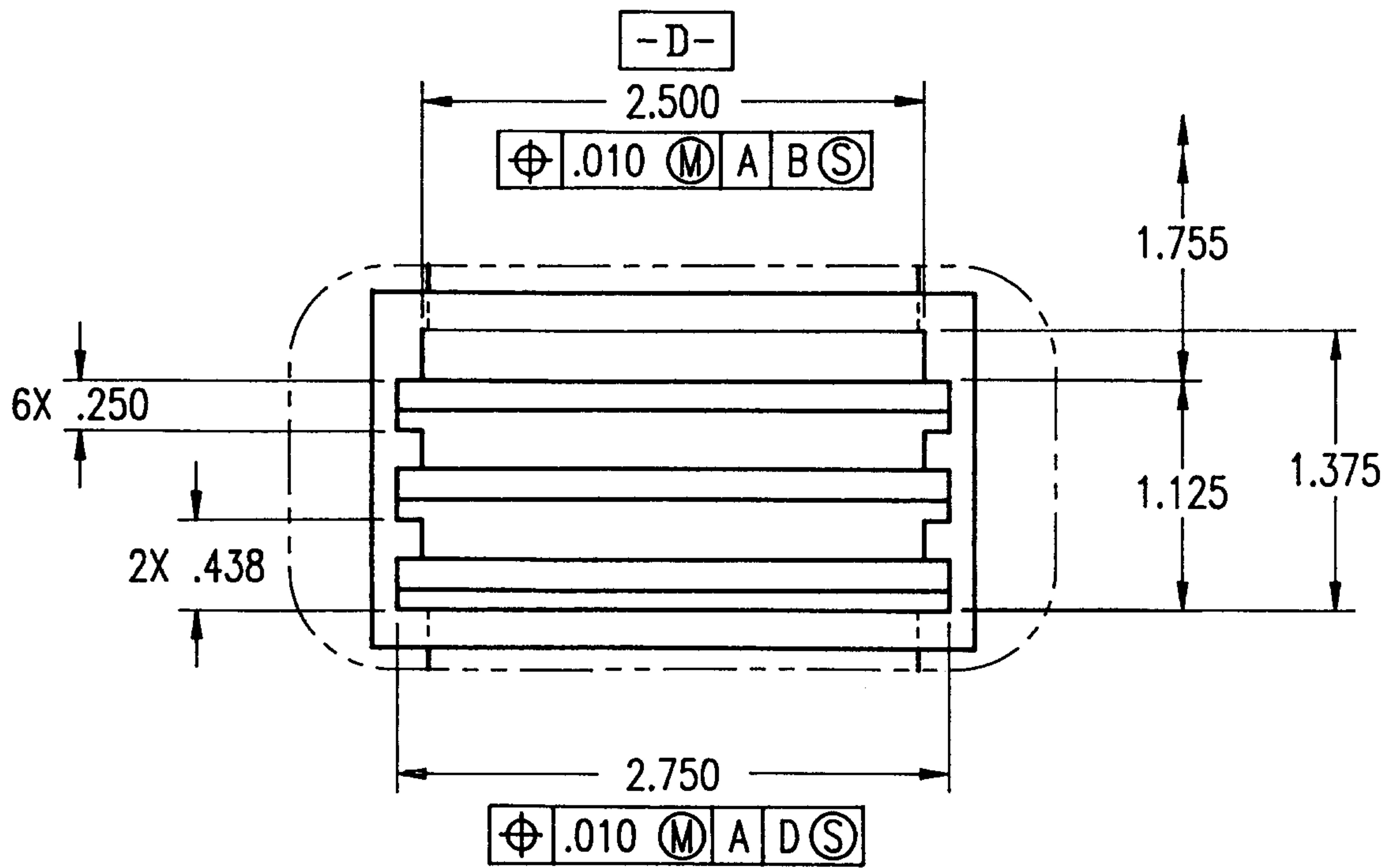
DETAIL C
