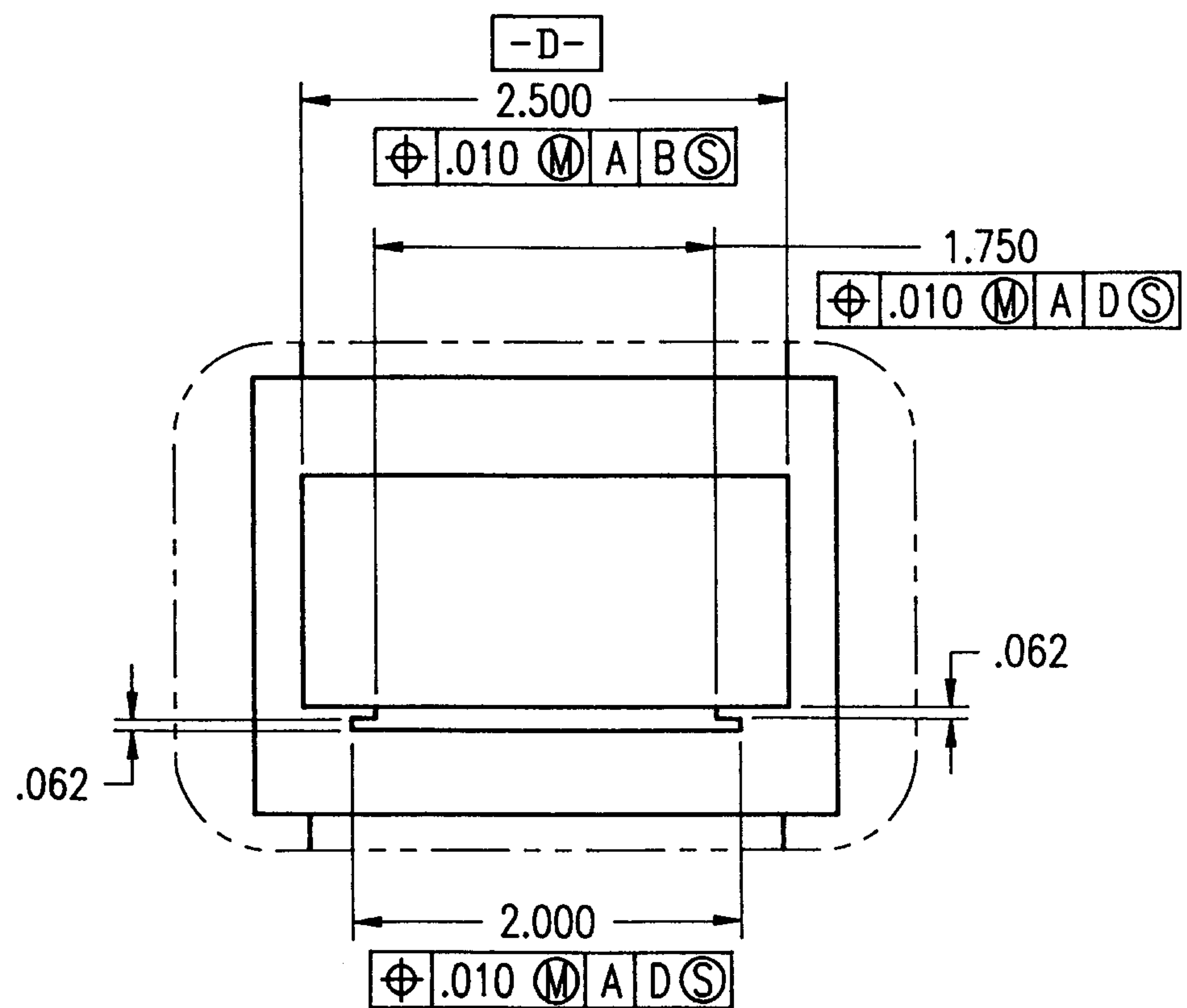
DETAIL B
