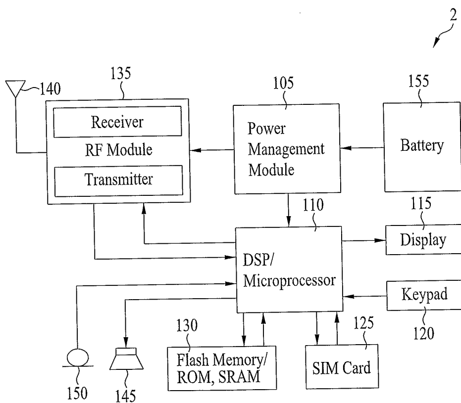
FIG. 25 MOBILE STATION/ACCESS TERMINAL
