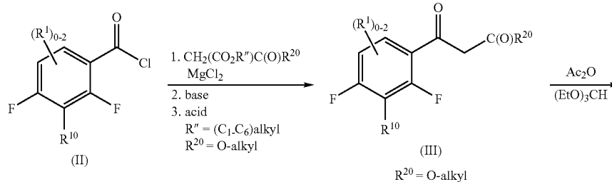
Reaction Scheme 1
