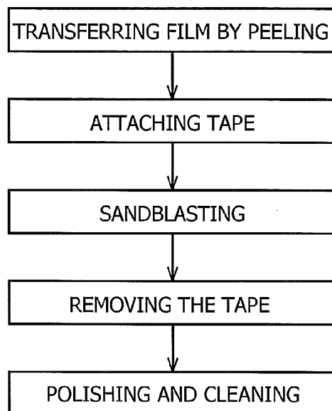
FIG.4 (RELATED ART)
