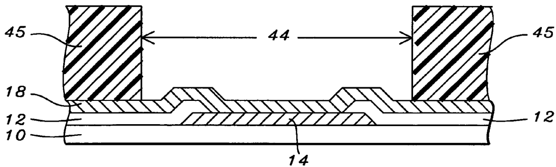
FIG. 14 - Prior Art
