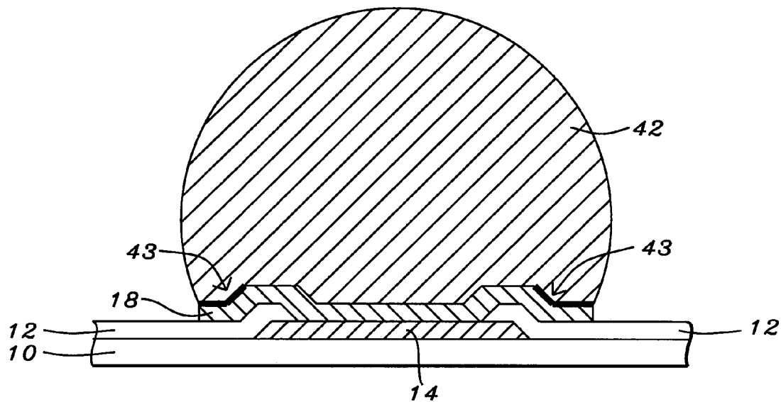
FIG. 13 - Prior Art
