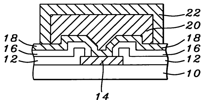
FIG. 3 - Prior Art
