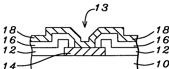
FIG. 2 - Prior Art
