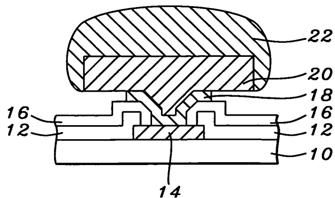
FIG. 4 - Prior Art
