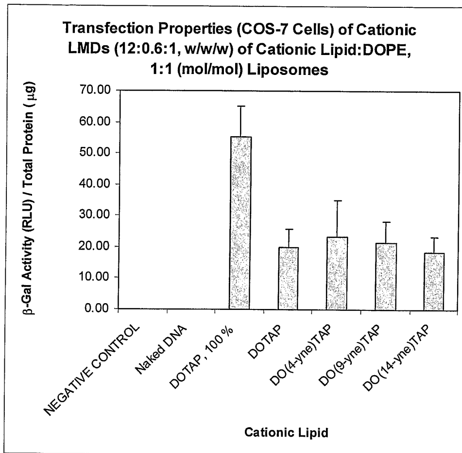
Figure 23: NB Transfast (not shown) 127 \pm 11 RLU / \mu g protein.
