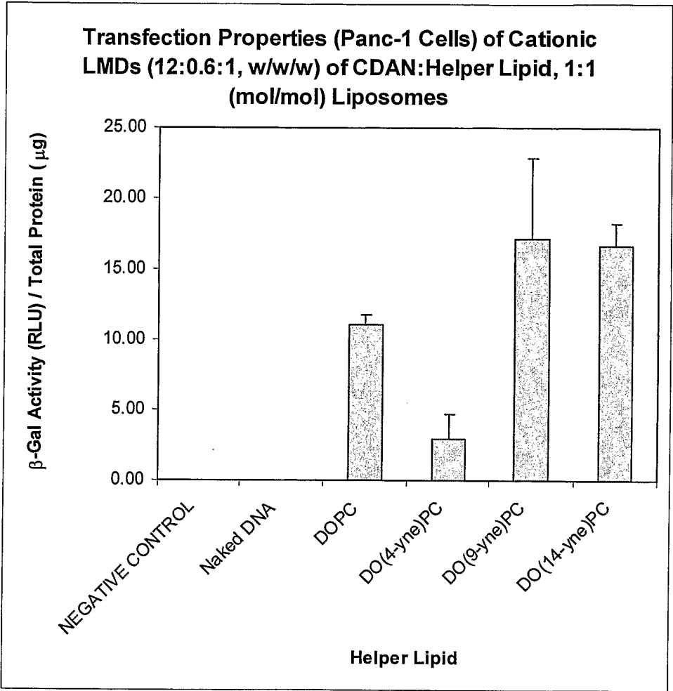
Figure 12: NB Transfast (not shown) 123 +/- 24 RLU / \mu g protein.
