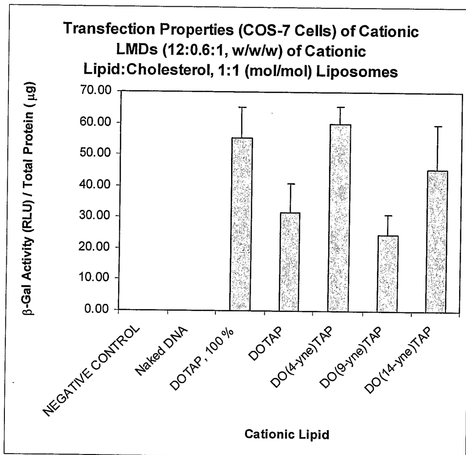
Figure 24: NB Transfast (not shown) 127 \pm 11 RLU / \mu g protein.
