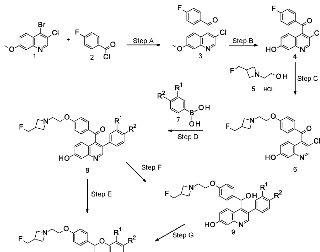
Scheme 1
