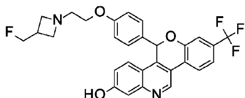
5-(4-{2-[3-(fluoromethyl)azetidin-1-yl]ethoxy}phenyl)-8-(trifluoromethyl)-5H-[1]benzopyrano[4,3-c]quinolin-2-ol;
