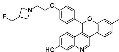
5-(4-{2-[3-(fluoromethyl)azetidin-1-yl]ethoxy}phenyl)-8-methyl-5H-[1]benzopyrano[4,3-c]quinolin-2-ol; and
