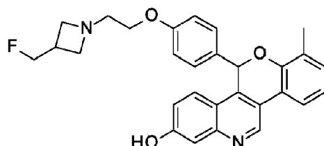
5-(4-{2-[3-(fluoromethyl)azetidin-1-yl]ethoxy}phenyl)-7-methyl-5H-[1]benzopyrano[4,3-c]quinolin-2-ol. -
