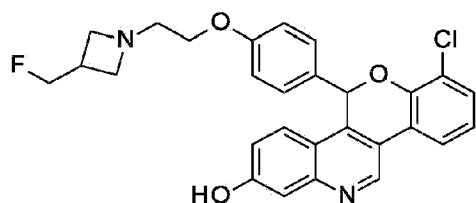
7-chloro-5-(4-{2-[3-(fluoromethyl)azetidin-1-yl]ethoxy}phenyl)-5H-[1]benzopyrano[4,3-c]quinolin-2-ol; -
