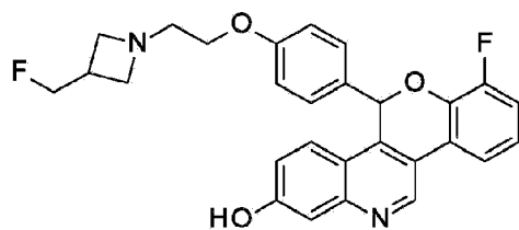
7-fluoro-5-(4-{2-[3-(fluoromethyl)azetidin-1-yl]ethoxy}phenyl)-5H-[1]benzopyrano[4,3-c]quinolin-2-ol; -
