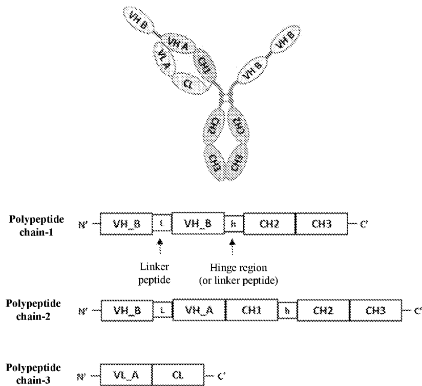
VH 1 HC-Fab-Fc-Dual VH
