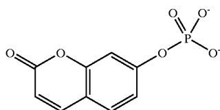
Umbelliferyl phosphate
