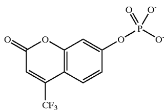
4-Trifluoromethylumbelliferyl phosphate
