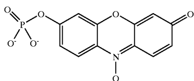
Resazurin phosphate
