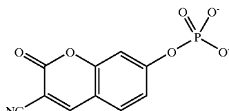
3-Cyanoumbelliferyl phosphate
