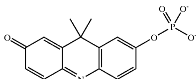
9,9-dimethylacridin-2-one-7-yl phosphate
