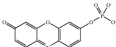
Resorufin phosphate
