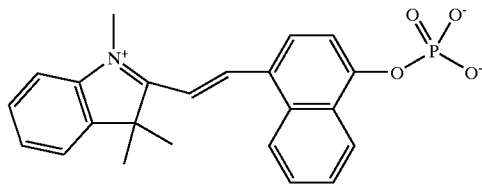
1-Ethyl-2-(naphthyl-1-vinylene)-3,3-dimethyl-indolinium phosphate
