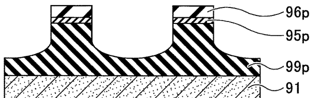
FIG.15D ETCH MIXED FILM
