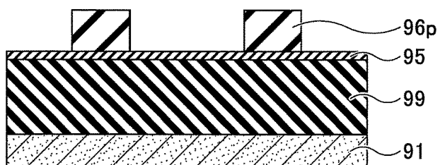
FIG.15C FORM RESIST PATTERN
