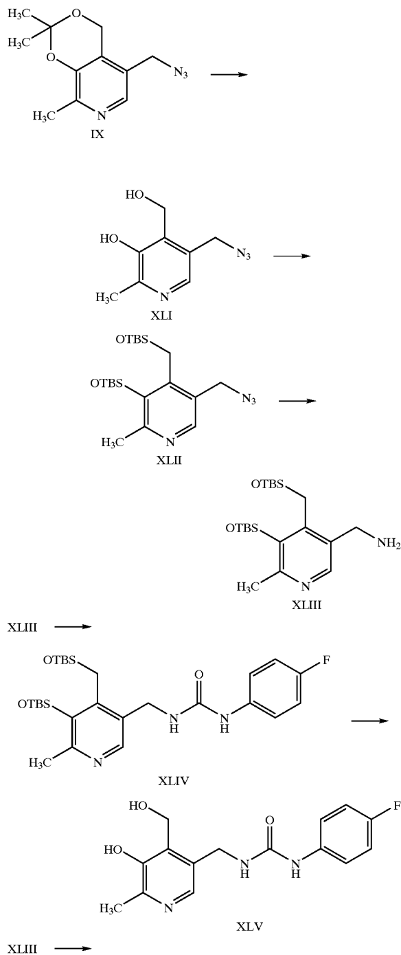
Scheme 5
