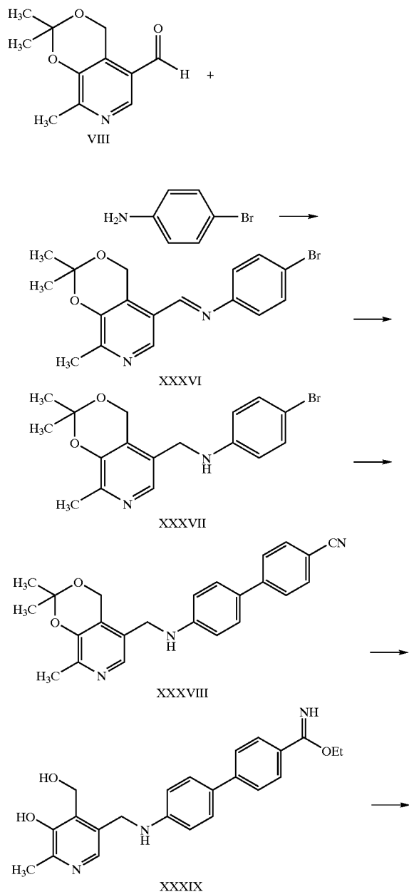
Scheme 12
