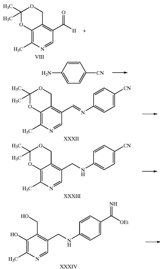
Scheme 3
