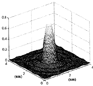
No Aberration FIG. 5A
