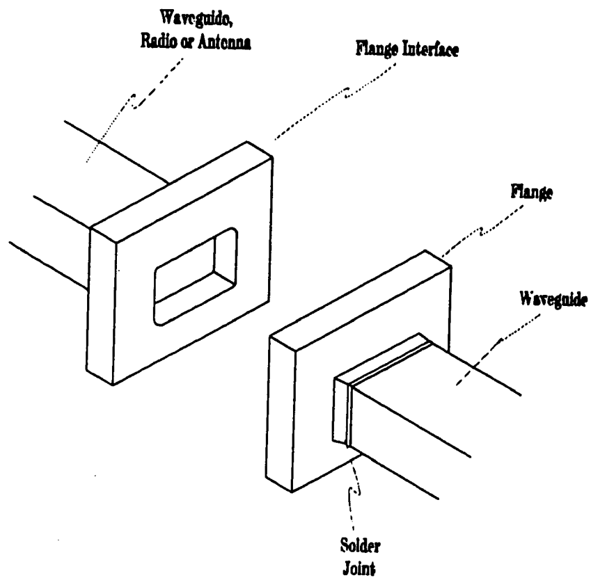
FIG. 9 (PRIOR ART)
