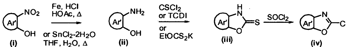
Scheme V
