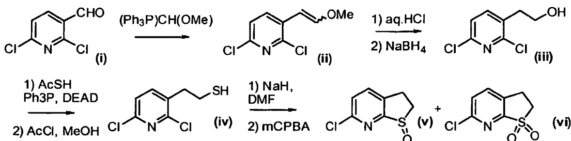
Scheme IV
