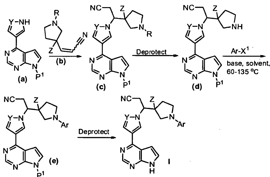
Scheme I
