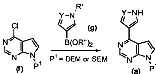
Scheme II
