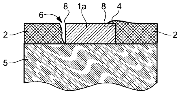
Fig. 1C ( Prior art )
