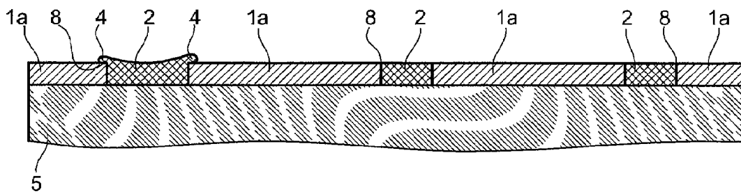
Fig. 2 ( Prior art )
