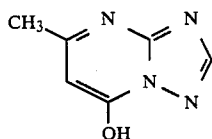
Structural formula of Compound (A)
