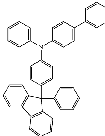
Step 1: synthesis method of 9-(4-bromophenyl)-9-phenylfluorene
