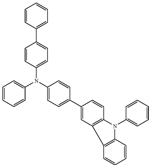
Step 1: synthesis method of 3-(4-bromophenyl)-9-phenyl-9H-carbazole
