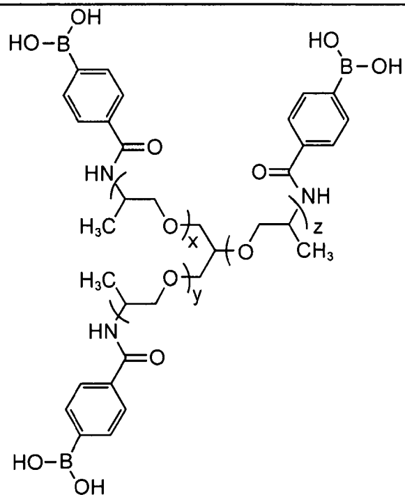
5: Polypropyletheramine-tricarboxyphenyl boronic acid (PPO-triboronic acid crosslinker)
