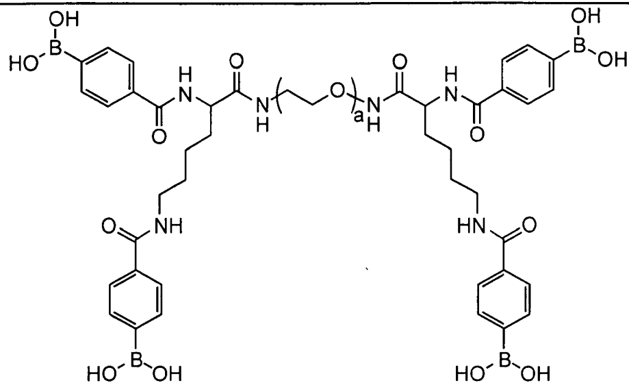
6: Bis-(amino-lysine-dicarboxyphenylboronic acid)-PEG (PEG-tetraboronic acid crosslinker)
