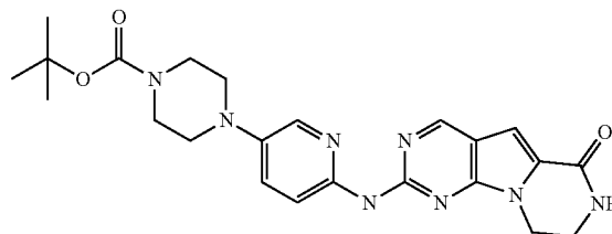
Compound 2
