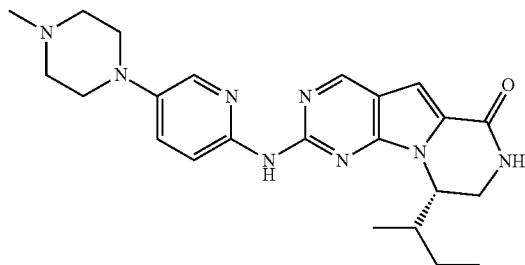
Compound 16
