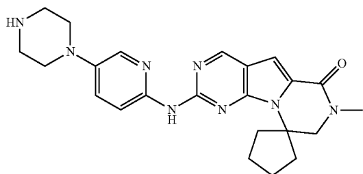
Compound 31
