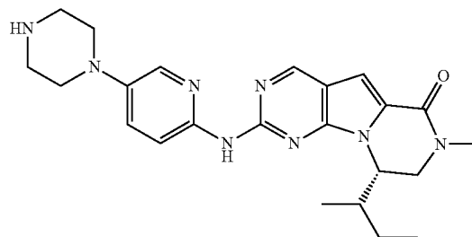
Compound 19
