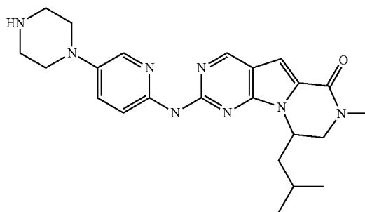
Compound 47
