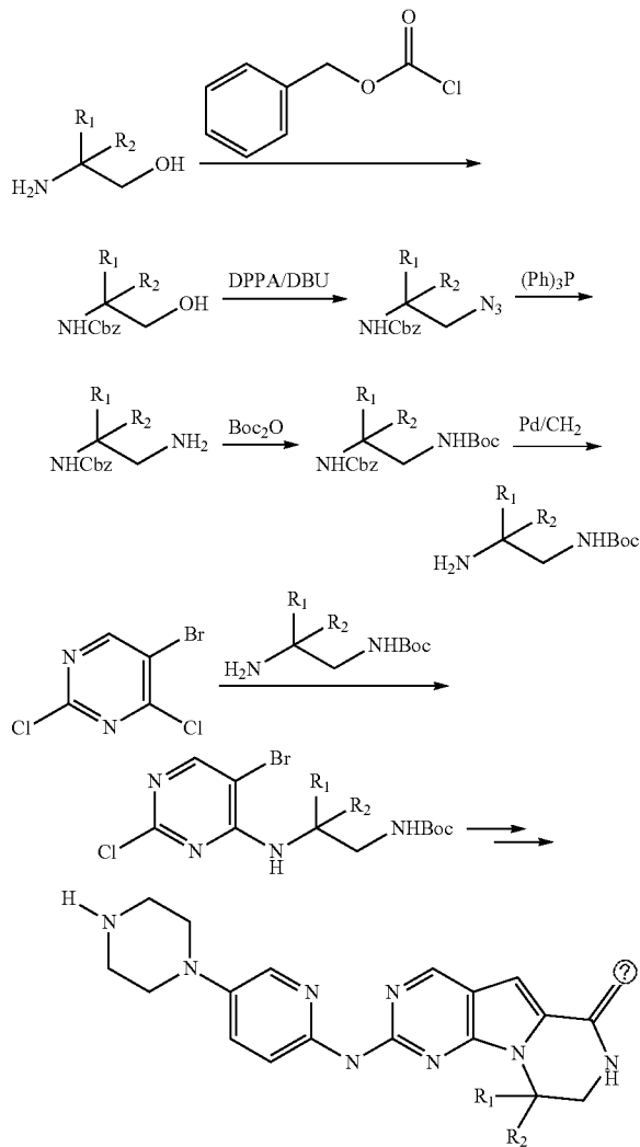
Scheme 4
