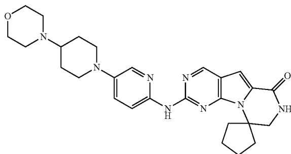
Compound 39
