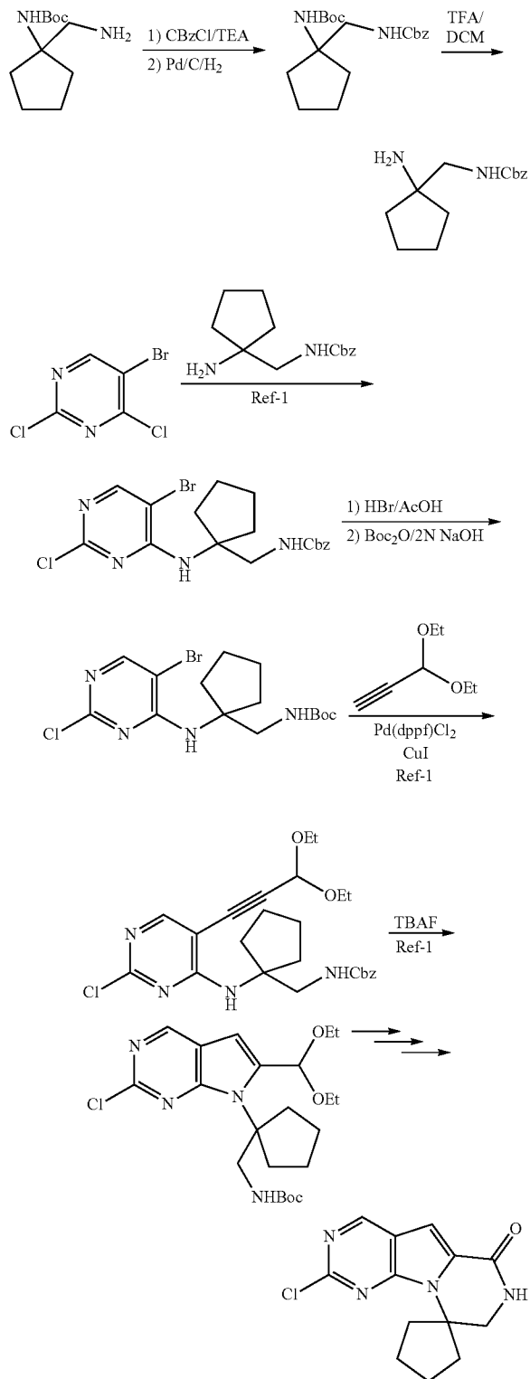
Scheme 3
