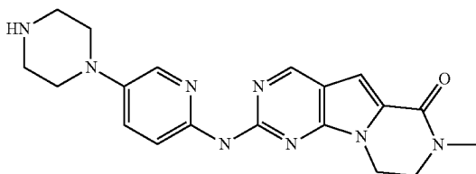
Compound 5
