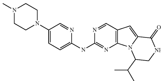
Compound 7
