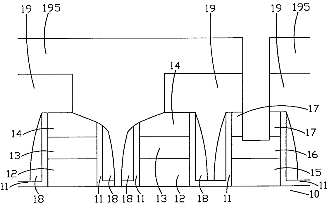
FIG.1C(Prior Art)
