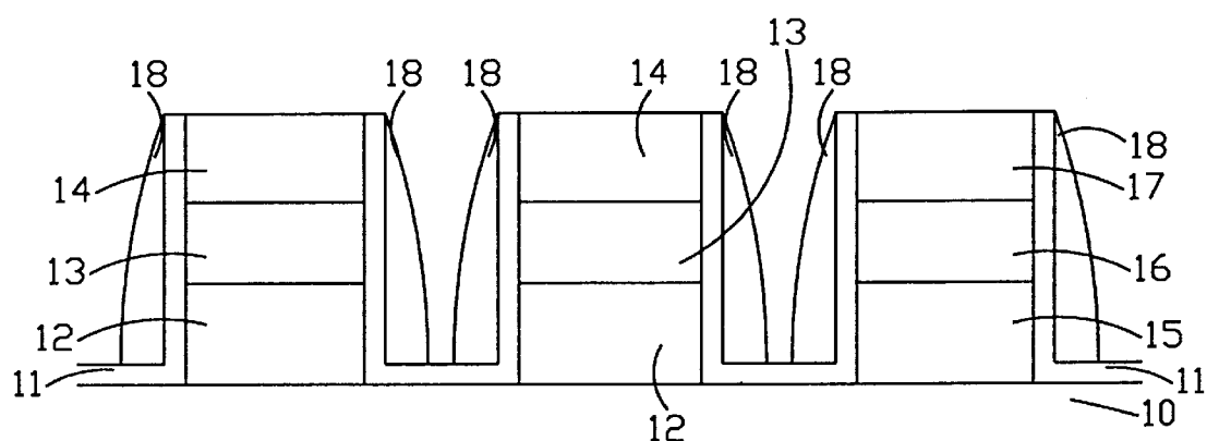
FIG.1A(Prior Art)
