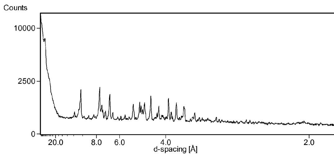
Figure 5: XRPD for Example 163 Free Base Crystalline Form A
