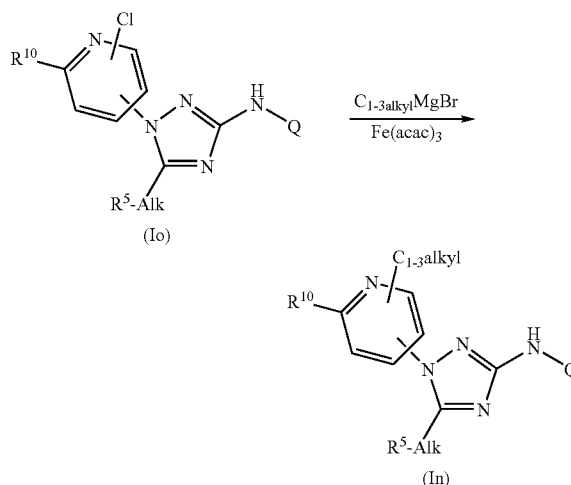
Scheme 12
