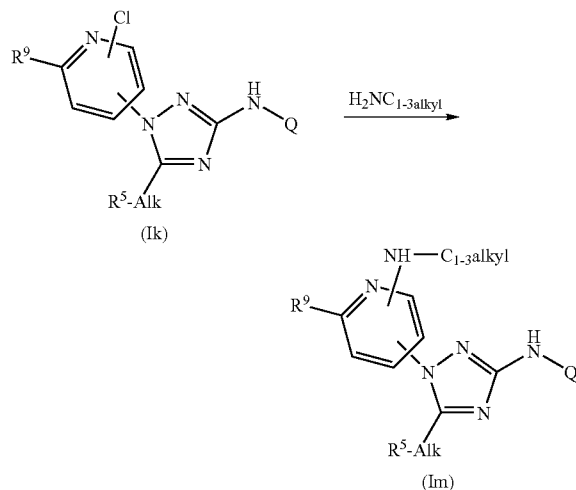
Scheme 11
