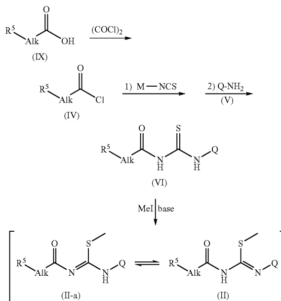
Scheme 2
