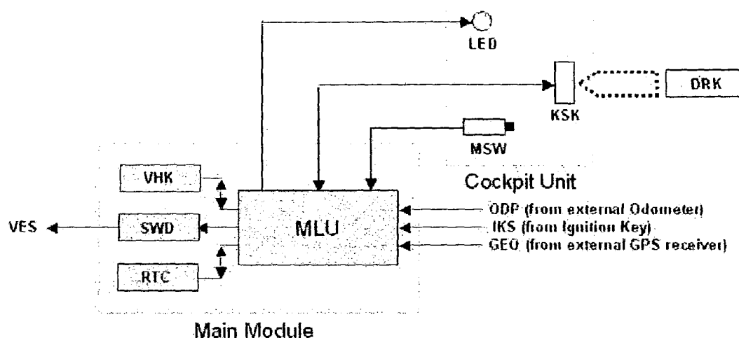
Figure 1 - Device for recording drive and journey data of motor vehicles
